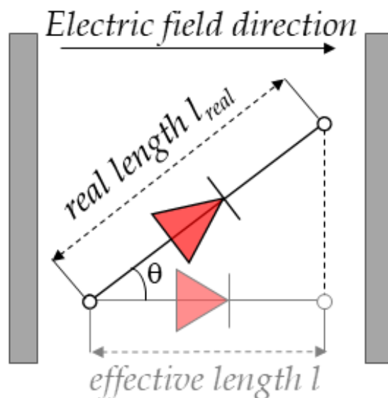
Scheme 1: Effective length of the LED in the direction of the electric field. The LED is orientated with an angle \theta with respect to the electric field direction. The grey rectangles are the feeder electrodes (top view).
