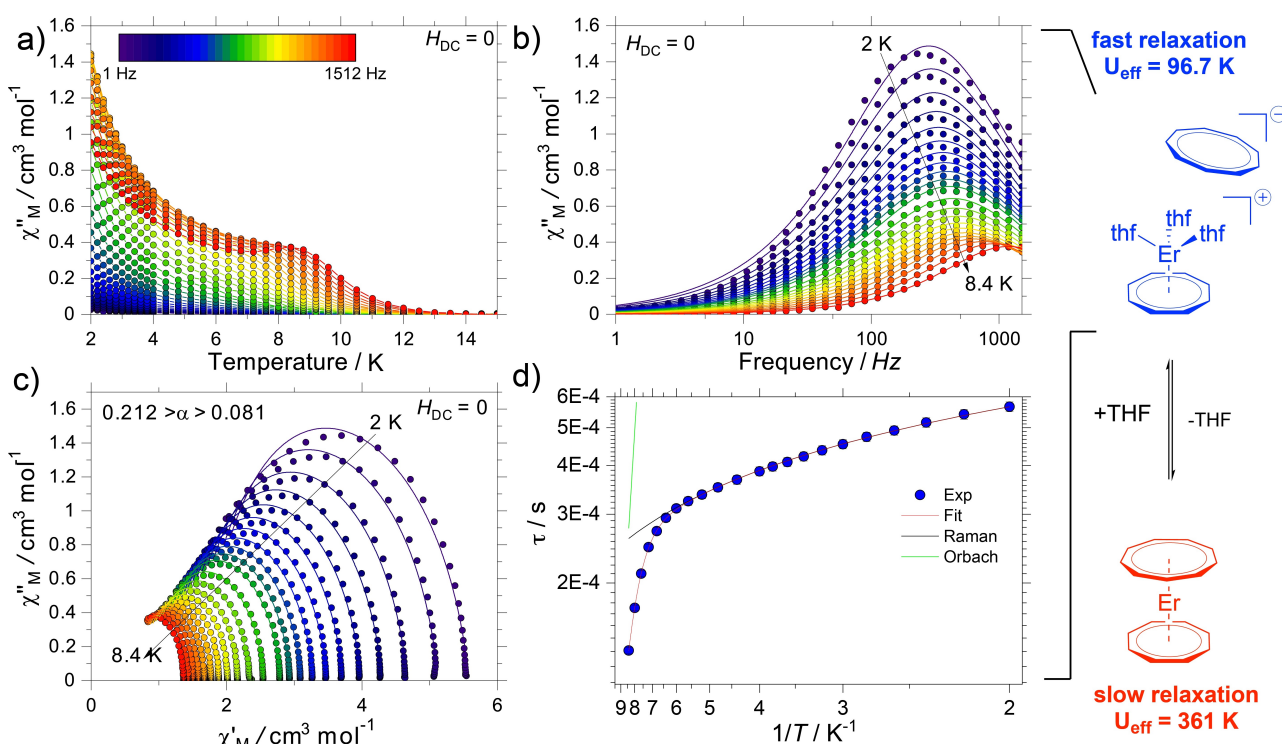
Figure 6. Dynamic magnetic data for the THF solvated complex 5 at zero field with an oscillating AC field of 3.5 Oe. a) \chi''_M(T) and b) \chi''_M(\nu) plots show the less efficient SMM properties compared to the unsolvated analogue [(\eta^9\text{-CNT})\text{Er}(\eta^8\text{-COT})] . Solid lines in panel (b) are fit to the generalised Debye model. c) Cole-Cole plots and distribution of relaxation times. d) Relaxation analysis for the obtained \tau . The relaxation data at zero field were fitted to \tau^{-1} = \tau_0^{-1} \exp(-\frac{U_{\text{eff}}}{kT}) + C\tau^n , with the best fit resulting in U_{\text{eff}} = 96.7(1) K, \tau_0 = 2.54(4) \times 10^{-9} s ^{-1} , C = 1214(6) s ^{-1} K ^{-n} , n = 0.541(3) .
