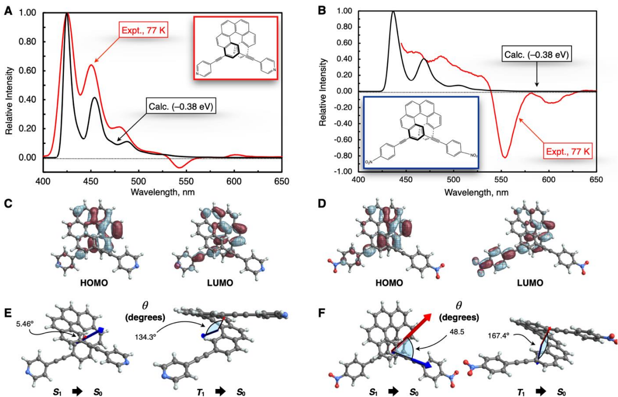
Figure 4. Calculated (black curves) and experimental (red curves) S_1 \rightarrow S_0 CPL spectrum of P -H6(py) 2 (left, panel A; the structure is shown in the red insert) and P -H6(NO 2 ) 2 (right, panel B; the structure is shown in the blue insert). Panels C and D show selected molecular orbitals of the U-DFT-optimized triplet excited state structure for both species ( \pm 0.03 isosurfaces). The molecular orbitals for the S_1 and S_0 structures are qualitatively similar (see Supporting Information). Panels E and F show electric (red arrows) and magnetic (blue arrows) transition dipole moments, arbitrarily scaled relative to the images of the U-DFT T_1 geometry, with the angle (in degrees) between them for the S_1 \rightarrow S_0 and T_1 \rightarrow S_0 transition, respectively.
