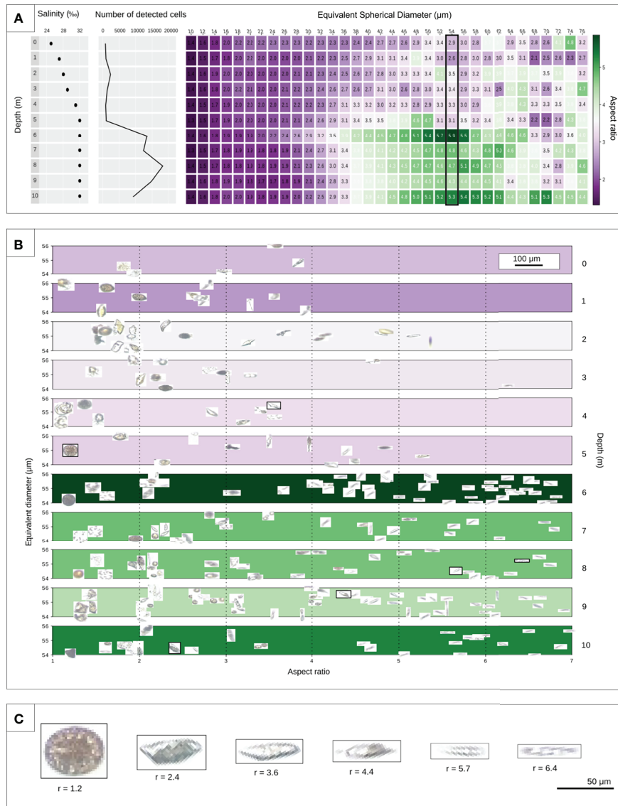
FIGURE 5 | PlanktoScope assessment of micro-plankton biodiversity along a vertical gradient in a Chilean fjord. (A) The extreme salinity gradient was measured in the Patagonian Comau fjord. Using sampling at discrete depths and the PlanktoScope, we attempted to describe correlations between salinity and plankton abundance/morphology across depths. Samples were collected with a Niskin bottle at different depths and imaged under a PlanktoScope. The plot depicts a vertical snapshot of an ecosystem from 0m (surface water) to 10m (depth) with the number of identified objects and equivalent diameter (10 to 76 \mu\text{m} ) as a function of depth (0 to 10m). The measurement of the elongation per equivalent diameter is based on 94,262 objects detected in total. Color bar represents the aspect ratio from purple (small aspect ratio) to green (large aspect ratio). (B) Display of distribution of objects with a mean size of 54 \mu\text{m} as a function of aspect ratio, equivalent diameter, and depths (0 to 10m). (C) Illustration of objects with a gradual aspect ratio from 1.2 to 6.4 marked in (B) .
