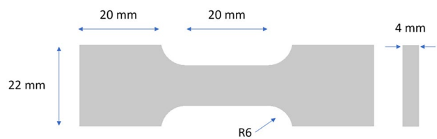
Fig. 1 Dimensions of specimen for tensile test
