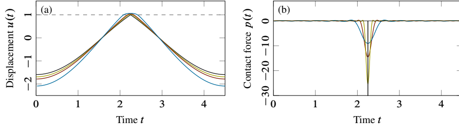
Figure A.5: Time-domain system response: (a) displacement, (b) contact force. Exact solution [—] and approximation with M = 10 [—], 20 [—], and 40 [—].
