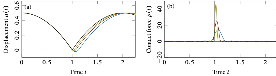
Figure A.2: Time-domain system response: (a) displacement, (b) contact force. Exact solution [—] and approximation with M = 10 [—], 20 [—] and 40 [—].
