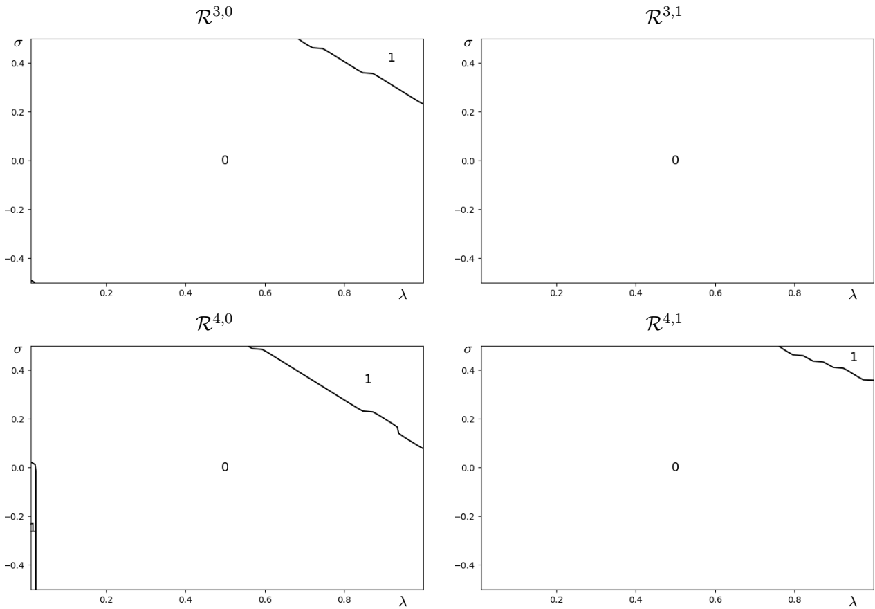
FIGURE 4. Number of zeros of the Kreiss-Lopatinskii determinant of O3 scheme with different reconstruction boundaries for \lambda \in ]0, 1[ and \sigma \in ]-0.5, 0.5[ .
