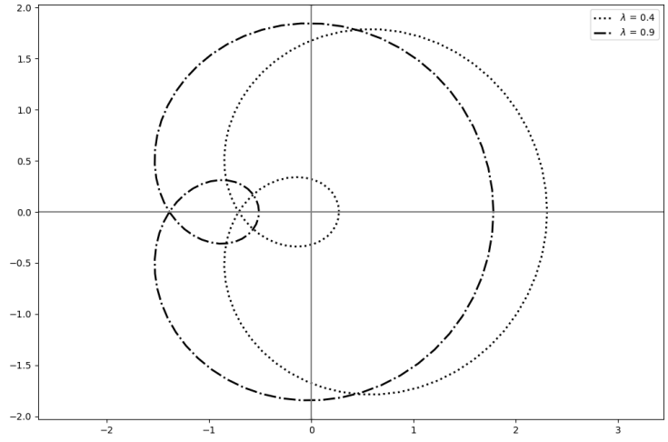
FIGURE 3. Curve \Delta(\mathbb{S}) for O3 scheme for \sigma = 0.4 , for \lambda \in \{0.4, 0.9\} with reconstruction boundary \mathcal{R}^{3,0} .
