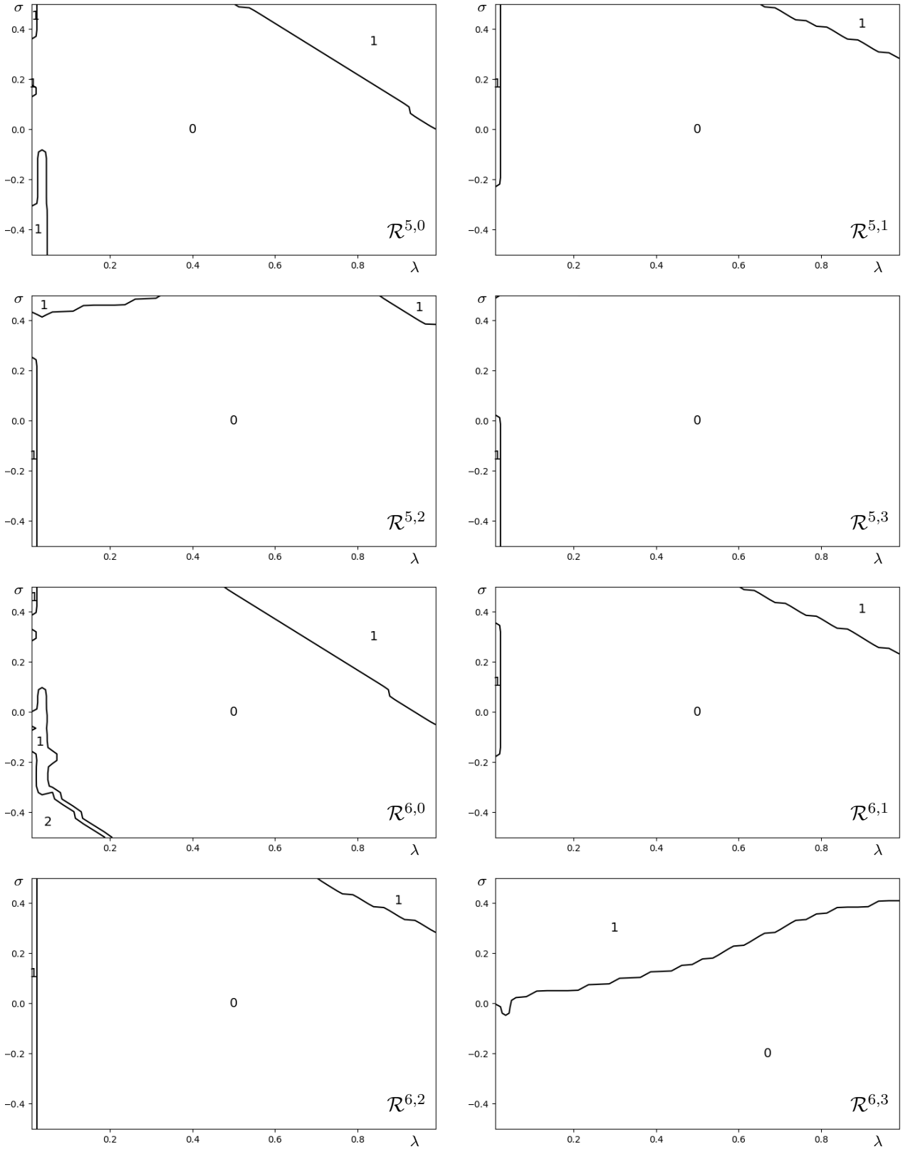
FIGURE 7. Number of zeros of the Kreiss-Lopatinski determinant of LW5 scheme with different reconstruction boundaries for \lambda \in ]0, 1[ and \sigma \in ]-0.5, 0.5[ .
