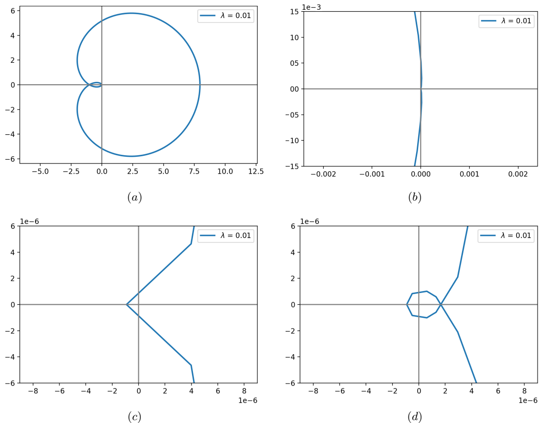
FIGURE 6. (a) representation of \Delta(S) for LW5 with the boundary condition \mathcal{R}^{6,1} , for \lambda = 0.01 and \sigma = 0 , zoom (b) without refinement (c) and with refinement (d).
