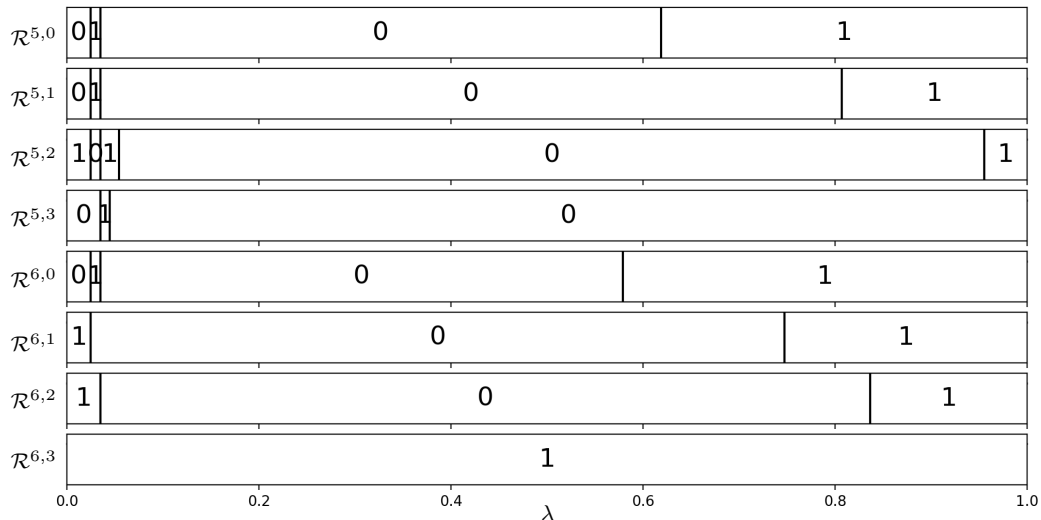
FIGURE 5. Number of zeros of the Kreiss-Lopatinskii determinant of LW5 scheme with different reconstruction boundaries for \lambda \in ]0, 1] and \sigma = 0.4 .
