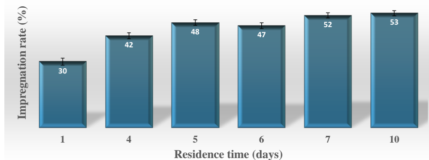
Fig. 4. Impregnation rate of hemp shives in CA as a function of time.
