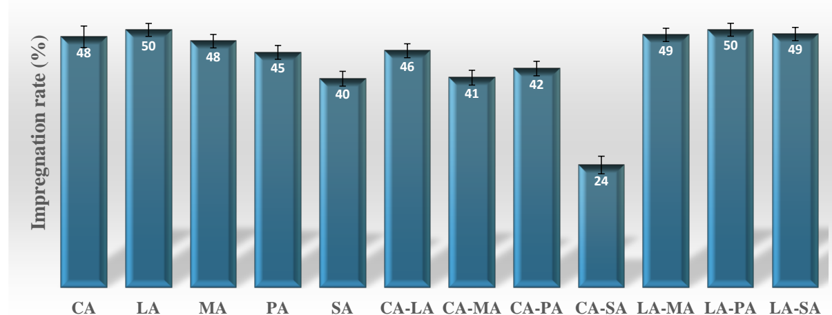
Fig. 7. Impregnation rate of hemp shives in fatty acids and their eutectic mixtures.
