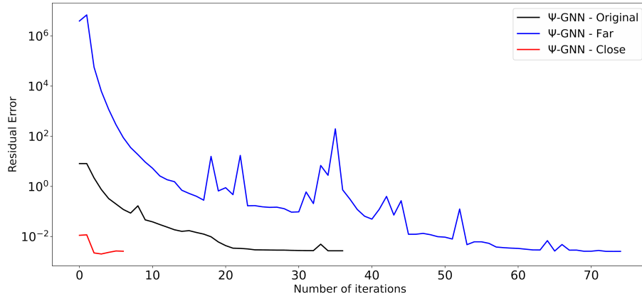
Figure 9: Evolution of the Residual error across iteration of \Psi -GNN for the same Poisson problem but considering three different initial solutions, demonstrating the adaptability of \Psi -GNN with respect to various initial solutions.
