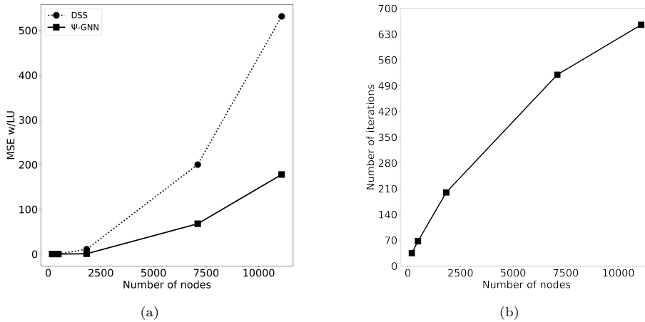
Figure 8: Figure 8a illustrates the averaged MSE w/LU for different mesh sizes for DSS, and \Psi -GNN. Figure 8b displays the averaged number of iterations performed by the Broyden solver in \Psi -GNN to reach its target threshold with respect to the number of nodes per mesh.
