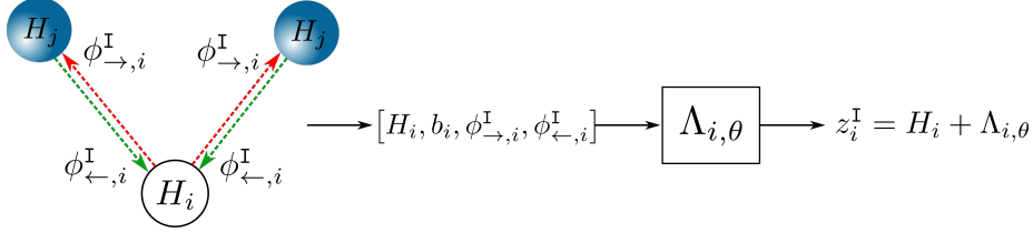
Figure 3: Process of updating the Interior latent variable z_i^I : Firstly, two MPNNs, \Phi_{\rightarrow,\theta}^I (red arrows) and \Phi_{\leftarrow,\theta}^I (green arrows), are computed to account for the bi-directionality of the edges. These computed messages are then concatenated with problem-specific data b_i and the actual latent state H_i and passed through a trainable function \Lambda_{i,\theta} . The output of this trainable function is finally used to calculate z_i^I in a Res-Net fashion.
