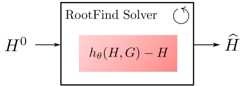
(c) \Psi -GNN : \hat{H} = \text{RootFind}(h_{\theta}(H, G) - H)
