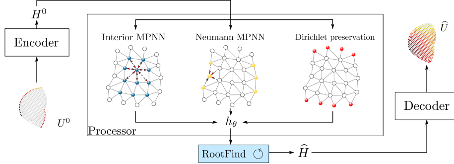
Figure 2: Diagram of \Psi -GNN: The model uses an Encode-Process-Decode architecture. The encoder maps an initial solution U^0 to some latent representation H^0 . The processor outputs a final latent state \hat{H} by considering a different treatment for each node type. Dirichlet nodes are preserved during the process, and specific MPNN (red arrows) for Interior and Neumann nodes are computed to build a GNN function h_\theta . A black-box “root-finding” solver automatically propagates the information through the graph by finding the fixed point \hat{H} of h_\theta , starting from the initial guess H^0 . The decoder maps \hat{H} back to the physical space to get the final solution \hat{U} .
