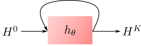
(b) Recurrent GNN : H^{k+1} = h_{\theta} (H^k)
