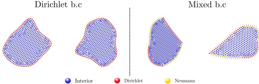
Figure 4: Geometries extracted from the synthetic dataset colored with respect to their node type (blue: Interior, red: Dirichlet, yellow: Neumann). These geometries are used to solve Poisson problems with Dirichlet boundary conditions only (on the left side) and mixed boundary conditions (on the right side). The arrows on the boundary of the two domains on the right represent the normal vectors.
