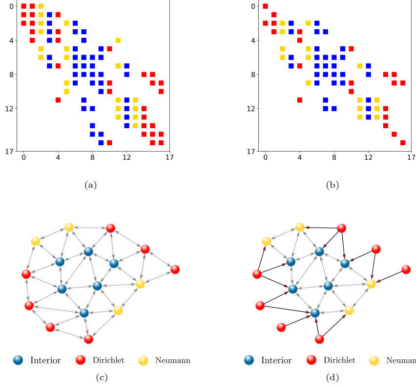
Figure 1: (1a) illustrates the sparsity pattern in matrix A , obtained by discretizing the Laplace operator in (1) using FEM for a problem with 17 nodes before applying Dirichlet boundary conditions. Using this matrix as an adjacency matrix, the induced graph is shown in (1c), resulting in a fully undirected graph. (1b) displays the sparsity pattern of the same matrix A after applying Dirichlet boundary conditions. The related graph is shown in (1d), resulting in an undirected graph for Interior and Neumann nodes (blue and yellow nodes) and a directed graph for Dirichlet nodes (red nodes). For both (1a) and (1b), Interior, Neumann and Dirichlet connections correspond to the blue, yellow and red squares, respectively.
