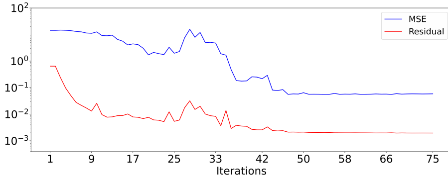
(d) Residual (red) and MSE w/LU (blue) losses
