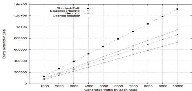
Figure 4. Maximum energy consumption (BS in the corner of a 10x10 grid)
