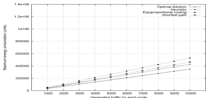
Figure 5. Maximum energy consumption (BS in the center of a 10x10 grid)
