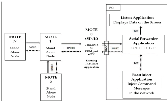
Figure 6. Communication Scheme
