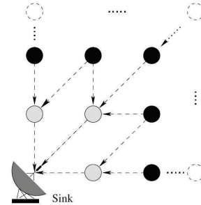
Figure 2. Shortest-Path strategy.
