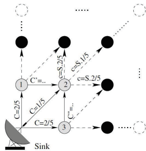
Figure 3. Contribution-Based Heuristic
