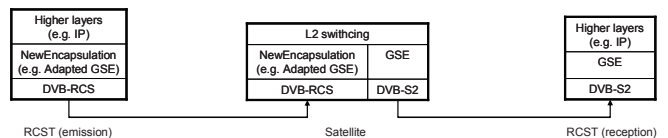
Figure 7: Protocol stacks for on board L2 switching
