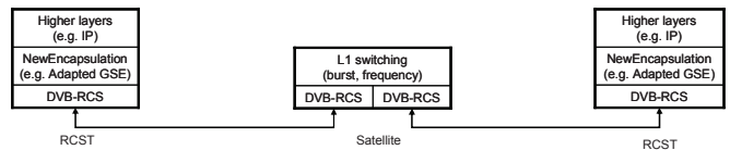
Figure 6: Protocol stacks for on board L1 switching
