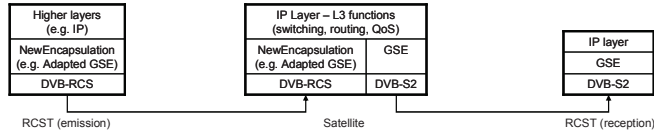
Figure 8: Protocol stacks for on board L3 switching
