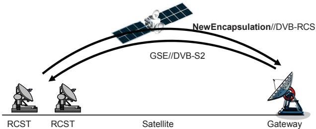
Figure 3: Forward and return link encapsulation
