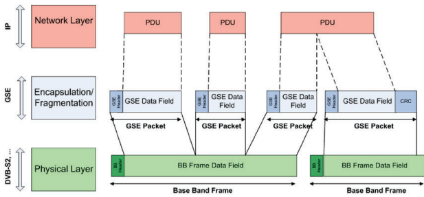
Figure 1: GSE encapsulation by DVB protocol stack [6]
