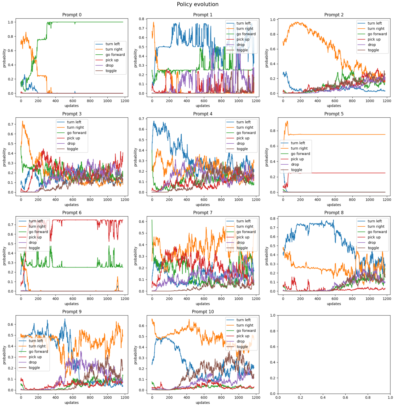
Figure 19. Evolution of actions' probability over training for test prompts listed in Table 2.
