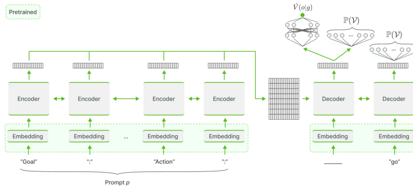
Figure 10. NPE-Flan-T5: We use the Flan-T5 architecture and add a value head. We initialize the embedding with the pretrained weights (framed in green in the diagram) and the other weights randomly. NPE-Flan-T5 stands for non-pretrained with pretrained embedding Flan-T5.
