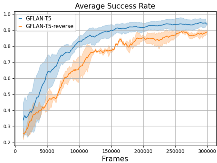
Figure 18. Comparison of the average success rate over training for GFLAN-T5 on the Go To when the actions “turn left” and “turn right” are flipped (“-reverse”). The success rate is given over 2 seeds with standard deviation.
