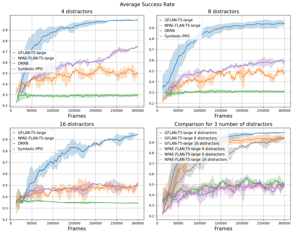
Figure 17. Learning curves for the agents on the Go To task for different number of distractors (4, 8, 16). The success rate is given over 2 seeds with standard deviation.
