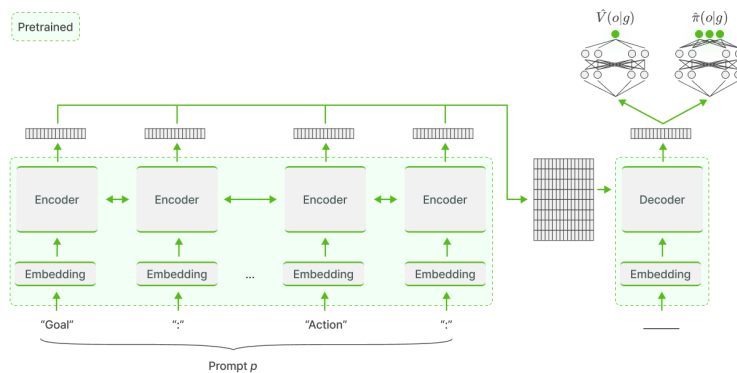
Figure 8. AFlan-T5: We use the Flan-T5 architecture but replace the language modeling heads with action heads (that return the probability for each action) and add a value head. We initialize the embedding, the encoder and decoder parts of the agent with the pretrained weights (framed in green in the diagram) and the other weights randomly. AFlan-T5 stands for action heads Flan-T5.
