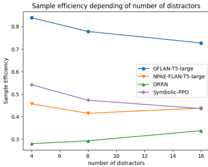
Figure 16. We measure the impact of the number of distractors on the sample efficiency measure (Equation (3)). We report results averaged over 2 seeds for training on the Go To task.
