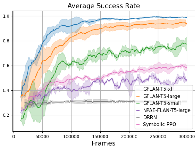
Figure 13. Impact of the size of the LLM on online RL finetuning. We conduct the tests with the Go to <object> task in 1 room, with 8 distractors. We measure the evolution of average success rate over 2 seeds with standard deviation for GFLan-T5 small (80 million parameters), GFLan-T5 large (780 million parameters) and GFLan-T5 XL (3 billion parameters). DRRN, NPAE-Flan-T5-large and Symbolic-PPO are given as baselines.
