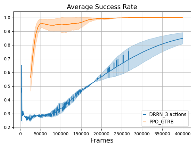
Figure 6. Average success rate for DRRN and Symbolic-PPO on the Go To Red Ball task with standard deviation over two random seeds. The PPO receives symbolic information and the DRRN gets textual observations.
