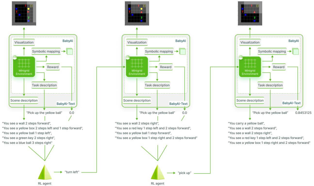
Figure 4. An illustration of how our BabyAI-Text environment encapsulates BabyAI. We keep the inner minigrid environment as well as task descriptions and reward but map the partial view of the agent to a text description.
