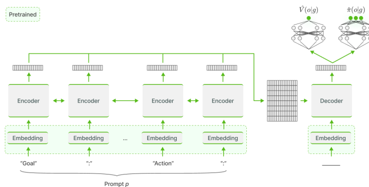
Figure 9. NPAE-Flan-T5: We use the Flan-T5 architecture but replace the language modeling heads with action heads and add a value head. We initialize the embedding with the pretrained weights (framed in green in the diagram) and the other weights randomly. NPAE-Flan-T5 stands for non-pretrained with action heads and pretrained embedding Flan-T5.
