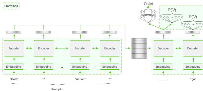
Figure 7. GFlan-T5: We use the Flan-T5 architecture and add a value head. We initialize the agent with the pretrained weights (framed in green in the diagram) including its language modeling heads to compute action probabilities. The weights of the value head are randomly initialized. GFlan-T5 stands for grounded Flan-T5.
