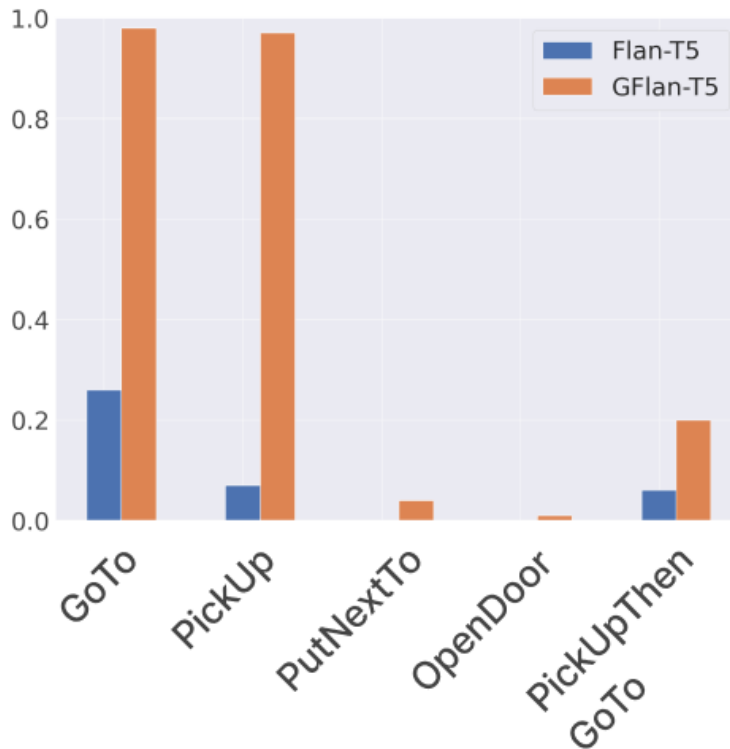
Figure 5. Per-task success rate for the 1000 evaluation trajectories performed in Figure 3.
