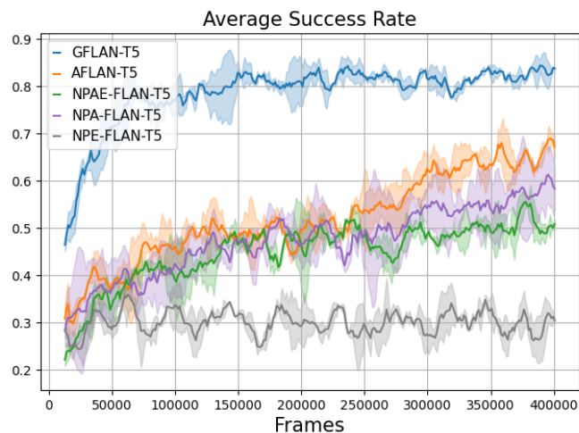
Figure 12. Average success rate of varying pretrained weights and scoring method with standard deviation over two random seeds. We train all LLMs on the Go to <object> task in 1 room, with 8 distractors, the 6 canonical actions and using Flan-T5 large (780 million parameters) as architecture.
