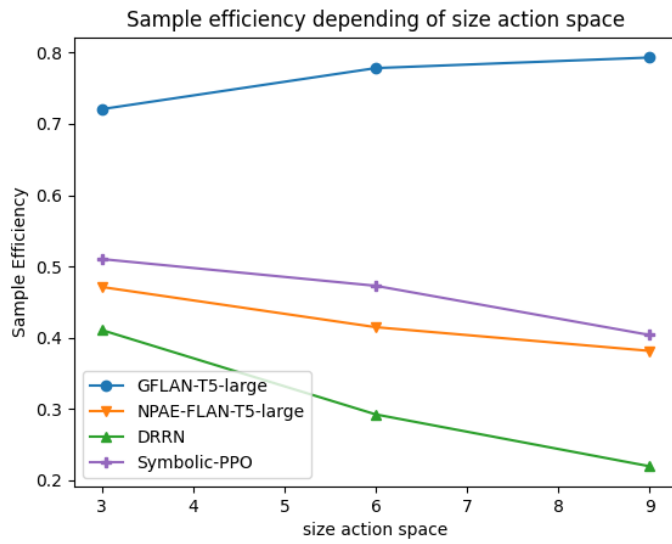
Figure 14. We measure the impact of the action space size (3, 6 or 9 actions with always only 3 useful actions) on the sample efficiency measure (Equation (3)). We report results averaged over 2 seeds for training on the Go To task.
