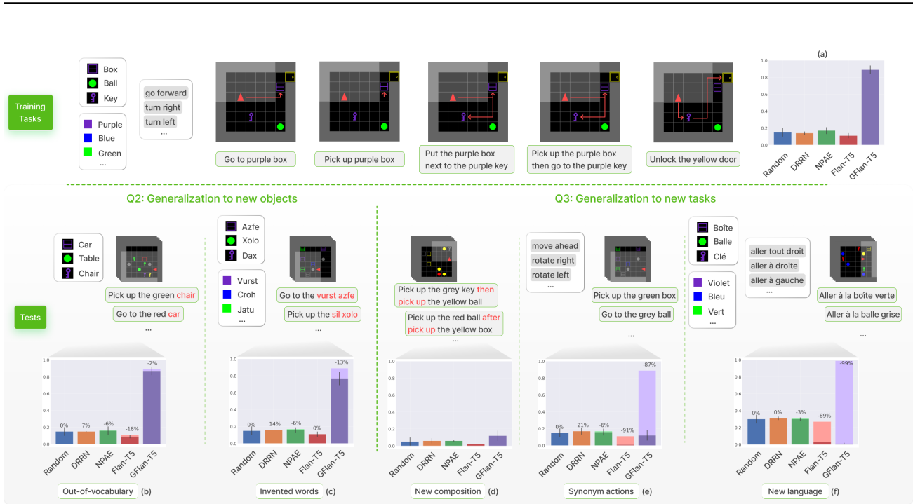
Figure 3. Generalization tests: We train all agents on a mix of 5 different tasks and evaluate their generalization abilities on 1000 test episodes (also containing a mix of these 5 tasks) (a). We compare them to two baselines: an agent choosing actions randomly (Random) and the zero-shot Flan-T5 (without any finetuning). We then perform several generalization studies to answer Q2 and Q3 by (b) substituting object names out-of-vocabulary names, (c) substituting objects and colors by invented words, (d) testing a new composition of tasks, (e) substituting actions by synonyms and (f) translating the whole environment to French for the Go To task. For each agent, we plot its mean success rate over 2 seeds along with the confidence interval and the delta with performance on the same task without any change (except for (d), on which no baseline result can be provided as this task is completely new).
