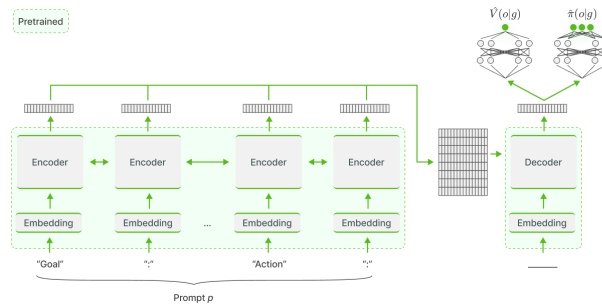
Figure 9: AFlan-T5: We use the Flan-T5 architecture but replace the language modeling heads with action heads (that return the probability for each action) and add a value head. We initialize the embedding, the encoder and decoder parts of the agent with the pretrained weights (framed in green in the diagram) and the other weights randomly. AFlan-T5 stands for action heads Flan-T5.
