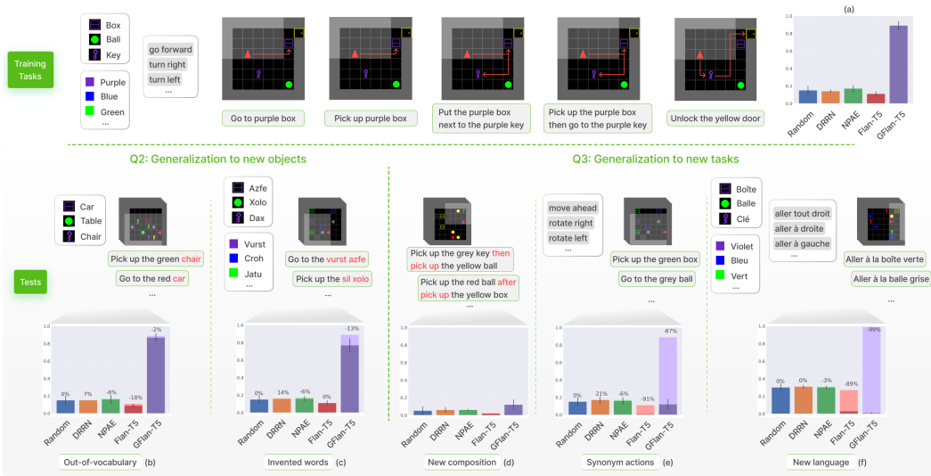
Figure 4: Generalization tests: We train all agents on a mix of 5 different tasks and evaluate their generalization abilities on 1000 test episodes (also containing a mix of these 5 tasks) (a). We compare them to two baselines: an agent choosing actions randomly (Random) and the zero-shot Flan-T5 (without any finetuning). We then perform several generalization studies to answer Q2 and Q3 by (b) substituting object names out-of-vocabulary names, (c) substituting objects and colors by invented words, (d) testing a new composition of tasks, (e) substituting actions by synonyms and (f) translating the whole environment to French for the Go To task. For each agent, we plot its mean success rate over 2 seeds along with the confidence interval and the delta with performance on the same task without any change (except for (d), on which no baseline result can be provided as this task is completely new).
