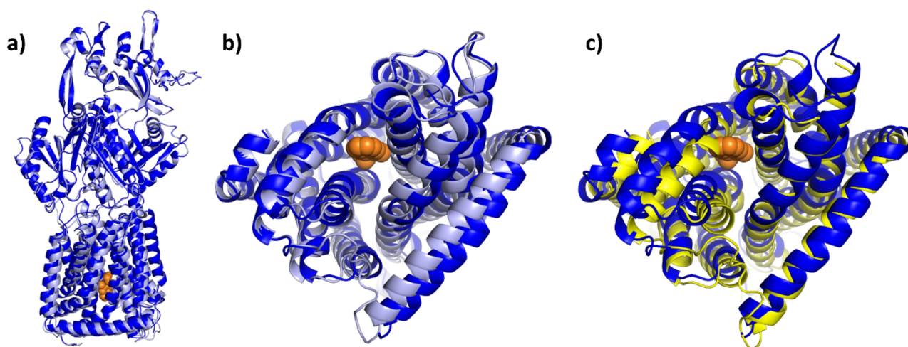
Figure 15. BDM88855-bound intermediate in comparison to the native AcrB L and T state. Cartoon models of the BDM88855 (shown as orange spheres) bound L-state (7OUK) and the native L and T states of AcrB (both 4DX5) were overlaid via their FD domains (residues 181–272 and 724–812). As can be seen, the entire periplasmic domain of AcrB/BDM88855 (blue) remains in the native L state (light blue) (a), while there are significant changes in the TMD (b). These changes are particularly evident in shifts of the second (right) TMD repeat (helices 7–12), which increases the cytoplasmic pocket. The conformation of the second repeat in the inhibitor-bound structure most closely resembles that of the native T state shown in yellow (c).
