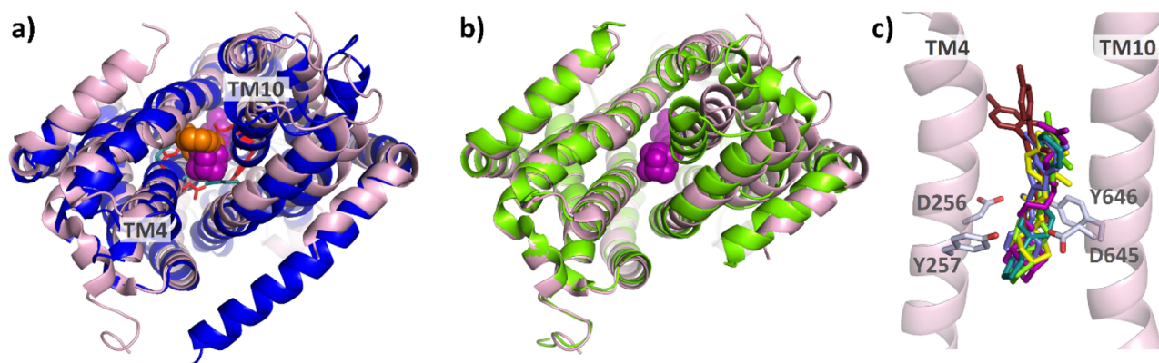
Figure 16. Comparison of AcrB/BDM88855 and inhibitor-bound co-structures of MmpL3: As can be seen from the bottom view (a) on the overlaid TMDs of AcrB/BDM88855 (7OUK) (blue/orange) and MmpL3/SQ109 (6AJG) (pink/magenta), both inhibitors bind to comparable areas within the respective proton relay networks (cyan and red sticks). A comparison of the inhibitor-bound MmpL3 co-structure and the native structure (6AJF) (green) shows that inhibition of MmpL3 is also associated with lateral shifts of the TMD repeats (b). The effects of MmpL3 inhibitors SQ109 (6AJG) (magenta), AU1235 (6AJH) (yellow), ICA38 (6AJJ) (light green), NITD-349 (7C2M) (light blue), SPIRO (7C2N) (teal), and rimonabant (6AJI) (brown) are likely all based on the disruption of the two Asp-Tyr pairs (D256, Y646 and D645, Y257) (c).
