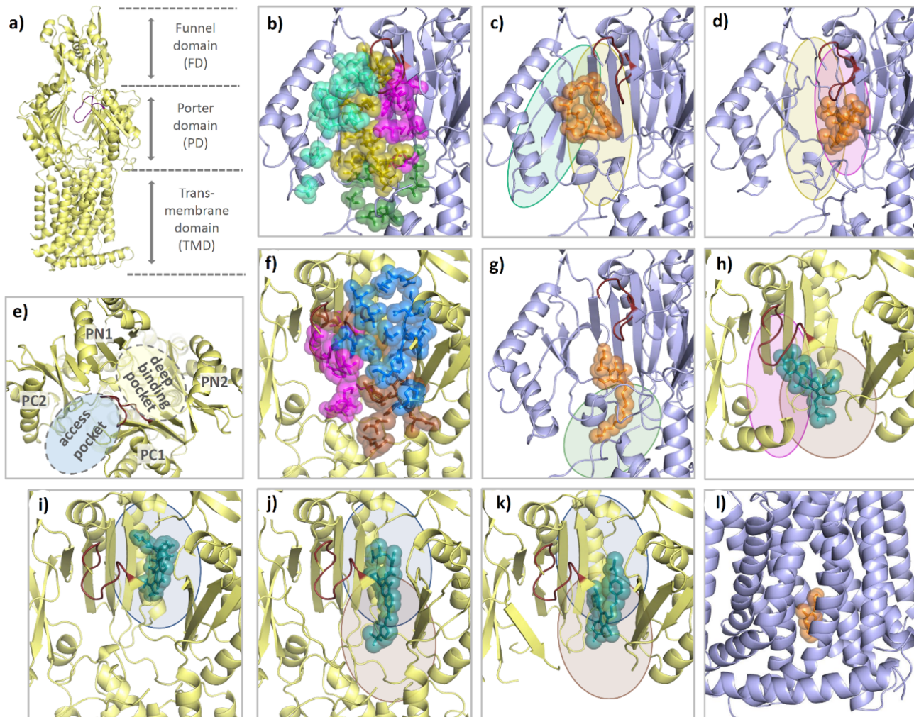
Figure 14. Comparison of the binding modes of AcrB substrates and inhibitors. Each AcrB protomer consists of a funnel domain (FD), a porter domain (PD), and a transmembrane domain (TMD) (a). The conformational states loose (L) and tight (T) are indicated by the color of the cartoon representation (light blue and yellow). As can be seen from a top perspective (e), the PD of the T protomer contains an access pocket (AP) and a deep binding pocket (DBP) that are separated by the switch loop (ruby). For the L protomer, all residues within 3.5 Å of a ligand are shown as colored spheres from a side perspective through the (removed) PC1 subdomain. Binding residues are grouped into an outer AP (cyan), an inner AP (olive), an AP-DBP interface (magenta), and channel 1 (CH1) (green) (b). As highlighted with the colors of the respective binding areas, the 3-formyl-rifamycin molecule (6ZOB) (shown as orange spheres, (c)), which is stalled in front of the switch loop, predominantly binds to the outer and inner AP. Erythromycin (3AOC) (d), which is located underneath the switch loop, is in close contact with the inner AP and the AP-DBP interface. DDM (6ZOA) was found in CH1 of an L/T intermediate (g). Main residues involved in T protomer substrate/inhibitor binding were grouped into an upper DBP groove region (blue), a lower DBP cave region (brown), and the residues of the AP-DBP interface (magenta) (f). While the binding of substrates (shown as teal spheres) such as fusidic acid (7B8S) (h) and minocycline (4DX5) (i) appears to focus on one of the two regions (and part of the AP-DBP interface), inhibitors such as D13-9001 (3W9H) (j) and MBX3132 (5ENQ) (k) interact strongly with both cave and groove of the DBP. The inhibitor BDM88855 (7OUK) (l) binds to a cytoplasmic pocket within the TMD of an early L/T intermediate.
