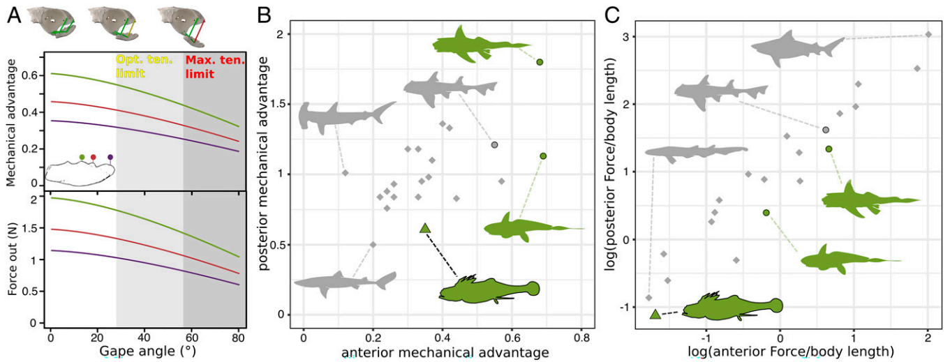
Fig. 3. Mechanical advantage and estimated output force in Inioperas , compared with extant chondrichthyans. (A) Mechanical advantage ( Top ) and estimated force out ( Bottom ) through the jaw closing cycle for Inioperas for three points along the inferred tooth row, namely, posterior (green), midpoint (red), and anterior (purple). Ranges for the optimal tension limit of the mandibular adductor and the maximum tension limit use the estimate based on a resting angle of 3 degrees. (B) Anterior vs. posterior mechanical advantage of the jaws of Inioperas compared with extant chondrichthyans. (C) Anterior vs. posterior estimated output force of the jaws of Inioperas compared with extant chondrichthyans, logged relative to body length. A key to B and C is as follows: gray points, elasmobranchs; green points, holocephalans; circles, durophages; diamonds, nondurophages; triangle, Inioperas . Silhouettes from Phylopic all under a Public Domain Mark 1.0 license: Scyliorhinus , uploaded by Birgit Lang; Squalus uploaded by M Kolmann; Hydrolagus and Chimaera , uncredited. Other silhouettes were made by Richard P. Dearden from images in Wikimedia Commons ( Carcharhinus and Sphyrna ) and from Zangerl and Case (16) ( Inioperas ). Abbreviations: ten., tension, otherwise as in Fig. 2.
