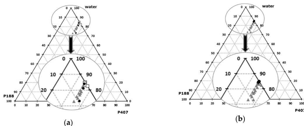
Figure 1. Ternary mix of Poloxamers 407/188 / H 2 O, sol-gel transition temperature (a), osmolarity (b).
