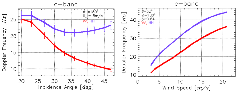
Fig. 9 Left: Simulated Doppler centroid anomaly (DCA) f_{dc}^{bias} (in Hz) as function of incidence angle for VV (red) and HH (blue) polarizations. The wind speed is fixed at 5 m/s and the radar look direction is upwind. The vertical bars reflect the variation in DCA with a change in wave age of 10%. Right: Simulated DCA as function of wind speed for VV (red) and HH (blue) polarizations at an incidence angle of 33 degrees. The radar look direction is supposed to be upwind
