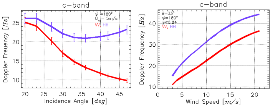
Fig. 9 Left: Simulated Doppler centroid anomaly (DCA) J_{dc}^{\text{bias}} (in Hz) as function of incidence angle for VV (red) and HH (blue) polarizations. The wind speed is fixed at 5 m/s and the radar look direction is upwind. The vertical bars reflect the variation in DCA with a change in wave age of 10%. Right: Simulated DCA as function of wind speed for VV (red) and HH (blue) polarizations at an incidence angle of 33 degrees. The radar look direction is supposed to be upwind
