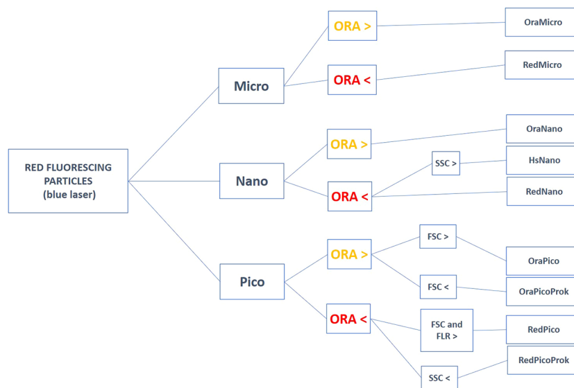
FIGURE 2 Decision tree for helping in the group's discrimination on cytograms for unstained natural red fluorescent particles excited with a blue laser. Red fluorescent particles corresponding to the phytoplankton groups are selected above a threshold that corresponds to the lowest limit of detection of the FCM. The lowest limit of detection is defined when the optical noise and the signature of the detritus in the sheath signal are well identified and do not affect the smallest resolved phytoplankton group the FCM can count (at best, the RedPicoProk). FSC= Forward scatter, FLR= Red fluorescence, FLO= Orange fluorescence, SSC= Sideward scatter. The groups RedRedPico and RedRedNano (discriminated with a red laser), as well as the HetHNA and HetLNA, are not presented here.
