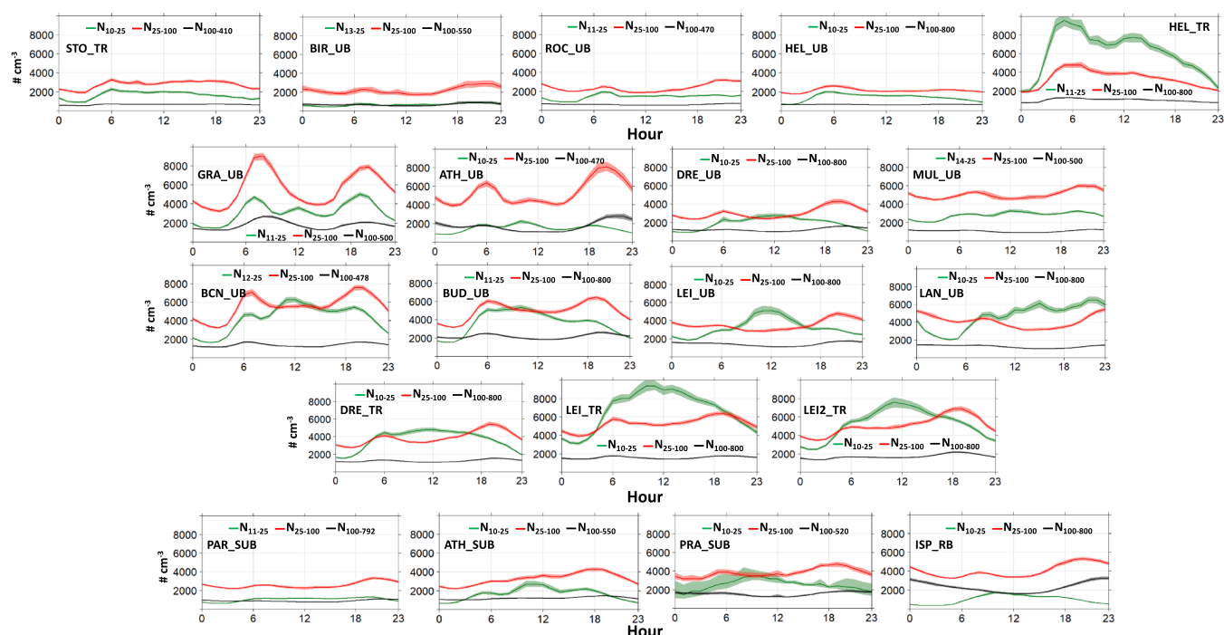
Fig. 5. Averaged 2017–2019 hourly concentrations of the particle number fractions (in \# \text{ cm}^{-3} ) N_{10-25} , N_{25-100} and N_{100-410} . Only sites with a lower size detection limit of 10–14 nm are included. UB, Urban background; TR, Traffic; SUB, Suburban background; RB, Regional background.
