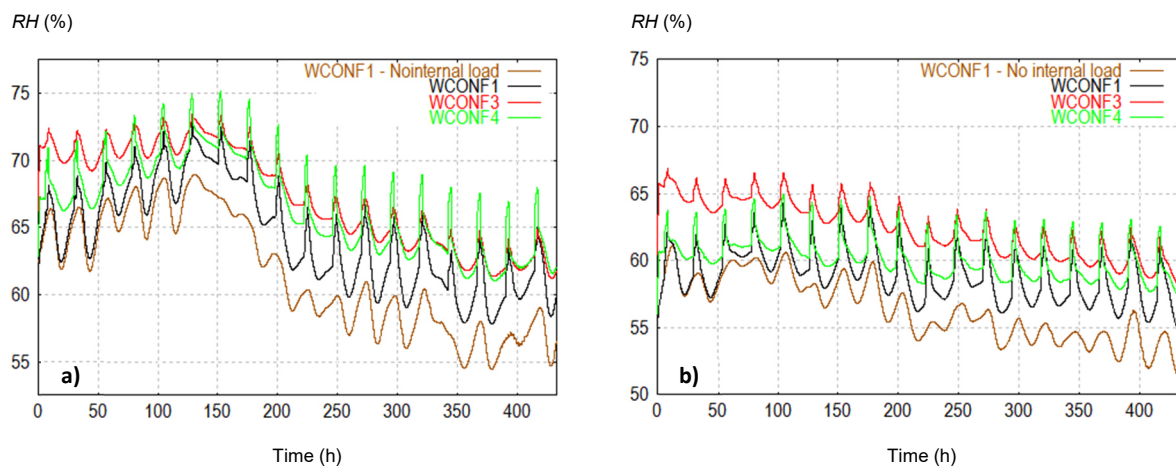
Figure 10: Temporal evolution of RH at Pos3 – TMCKIN / model (9) simulations with (a) Wroughton climate and (b) Bordeaux climate for the different wall configurations
