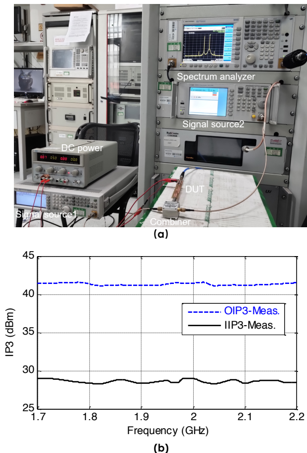
Fig. 7. OIP3 and IIP3 characterization (a) experimental setup and (b) measured results.
