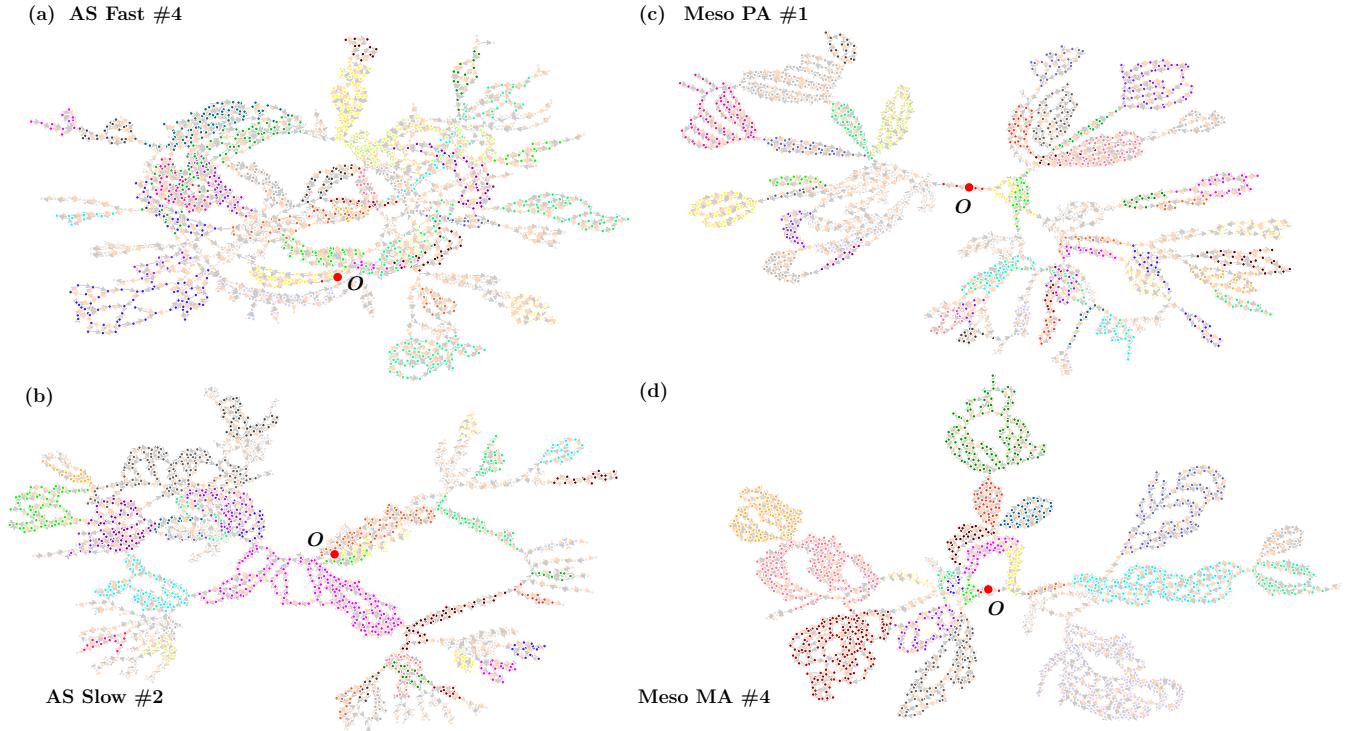
FIG. 9. Transition-graph representation of the AQS dynamics and thermal history – atomistic (AS) vs mesoscopic (Meso) models. Excerpts of transition graphs extracted from atomistic (a,b) and N = 32 mesoscopic glasses (c,d) with different thermal histories: (a,c) poorly-aged/fast quenched, (b,d) moderately aged/slow quenched. The color of each vertex indicates the strongly connected component (SCC) of the graph that it belongs to (refer to text for details) and the initial mesostate of the prepared glass has been marked with a larger red vertex labeled O . Vertices belonging to SCCs of size less than 10 have been colored in light gray.
