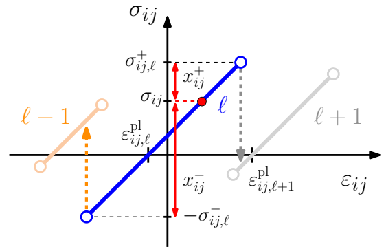
FIG. 1. Local elastic branches associated with a cell (i, j) . Each elastic branch \ell is characterized by a pair of stress thresholds \sigma_{ij,\ell}^{\pm} and a plastic strain \varepsilon_{ij,\ell}^{\text{pl}} , which prescribe the behavior of the local stress \sigma_{ij} under elastic strain \varepsilon_{ij}^{\text{el}} = \varepsilon_{ij} - \varepsilon_{ij}^{\text{pl}} , as shown for the branch labeled \ell in the figure. When the stress reaches the upper or lower stress threshold, a transition to the corresponding neighbouring branches, \ell \pm 1 occurs. The current stress state of the cell is denoted by a red filled symbol on the elastic branch \ell . This allows us to define the local plastic strengths x_{ij}^{+,\text{pl}} = \sigma_{ij}^{+} - \sigma_{ij} and x_{ij}^{-,\text{pl}} = \sigma_{ij}^{-} - \sigma_{ij} which give the distance to threshold in the forward and backward directions, respectively. The slopes of the local branches are identical and equal to 2\mu .
