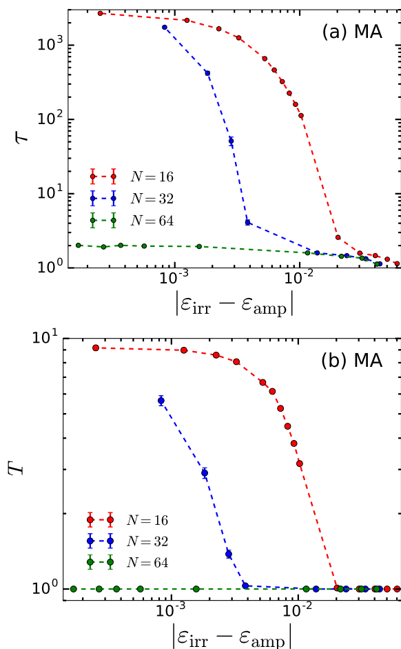
FIG. 8. Convergence to limit cycles of moderately-aged (MA) glasses: (a) Duration \tau of transients vs. relative cycle amplitude |\epsilon_{\text{irr}} - \epsilon_{\text{amp}}| , where \epsilon_{\text{irr}} is the system size dependent strain amplitude where the success-rate p_{\text{succ}} of cyclic response is 1/2 , cf. Fig. 6 (inset). (b) The period T of the cyclic response in units of driving cycles for the moderately-aged samples at different system sizes.
