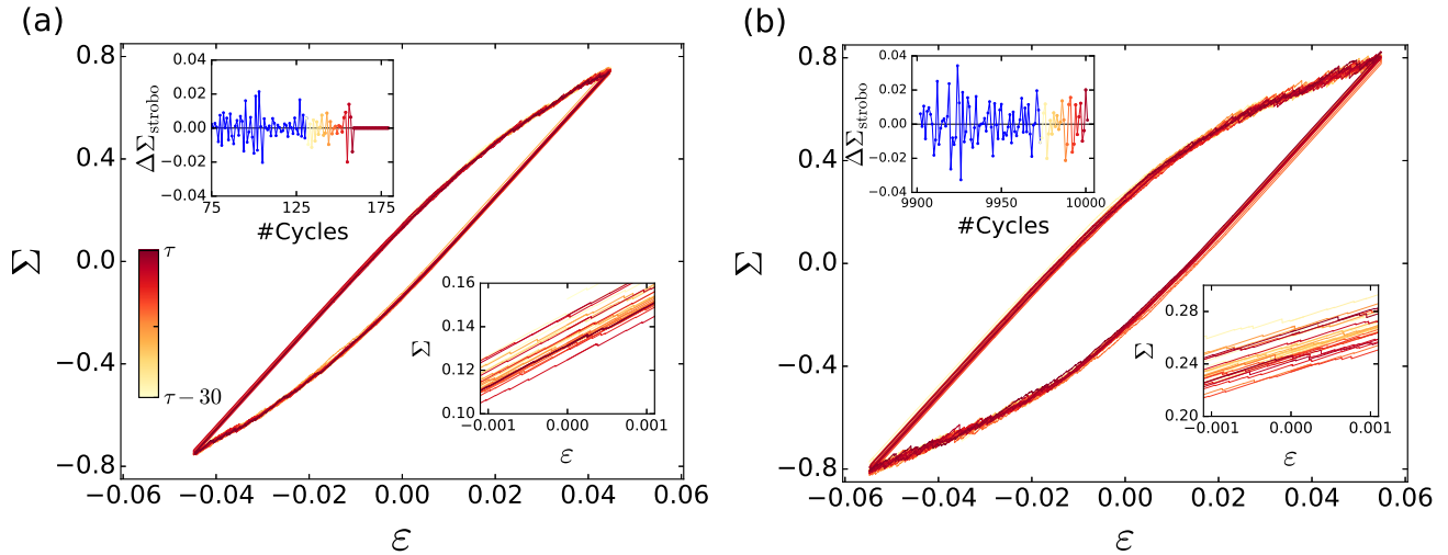
FIG. 5. Response of the N = 32 poorly-aged glass to cyclic shear at a strain amplitude below, (a) and above (b) the irreversibility transitions by \Delta \epsilon = 5 \times 10^{-3} . The main panels show the evolution of the stress-strain curve over the last 30 cycles with each subsequent cycle colored in a darker shade of red, as indicated in the legend. The insets to the lower right show a detail of this evolution. The insets in the upper left show the stroboscopic stress difference, obtained by taking the difference in stress at the beginning of two consecutive cycles, using the same coloring for the last 30 cycles. In (a) cyclic response is attained after a transient of \tau = 158 cycles, while in (b) such a response is still not obtained after 10^4 cycles.
