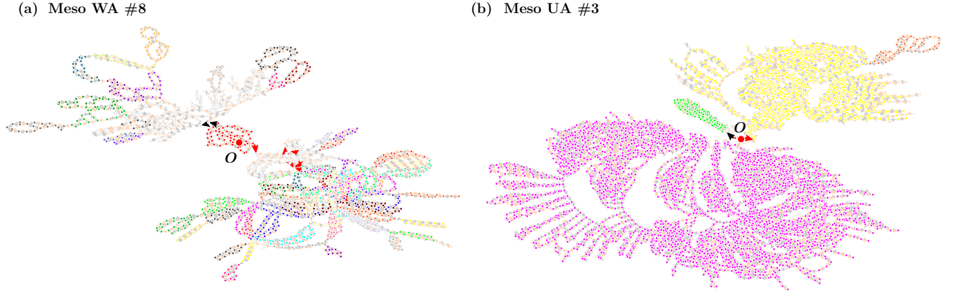
FIG. 15. Excerpts of transition graphs extracted from well-aged (WA) and ultra-well-aged (UA) mesoscopic glasses with N = 32 . Refer to text for further details.
