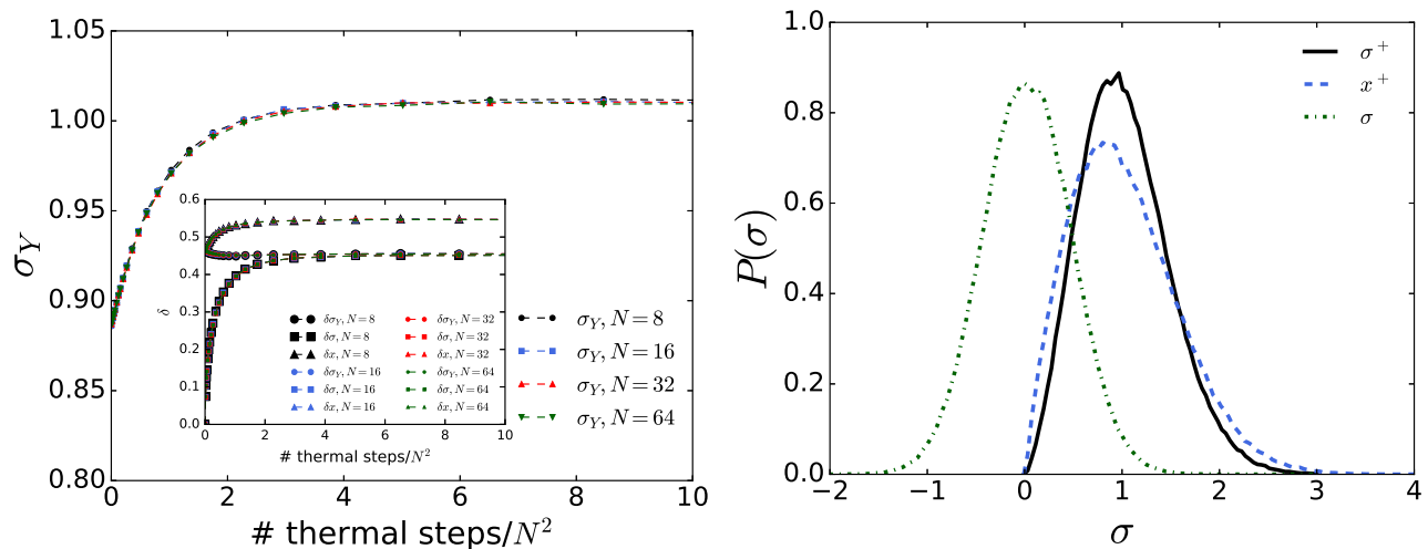
FIG. 2. Glass preparation - mimicking instant quench from high T: (a) evolution of the mean stress-threshold \overline{\sigma^+} with the number of (random) thermalization steps per site and for system sizes N = 16, 32 , and 64 . The inset shows the same evolution for the standard deviations of the stress thresholds \delta\sigma^+ , internal stresses \delta\sigma , and local plastic strength \delta x^+ . (b) stationary distributions of the fields \sigma , \sigma^+ and x^+ for N = 64 .
