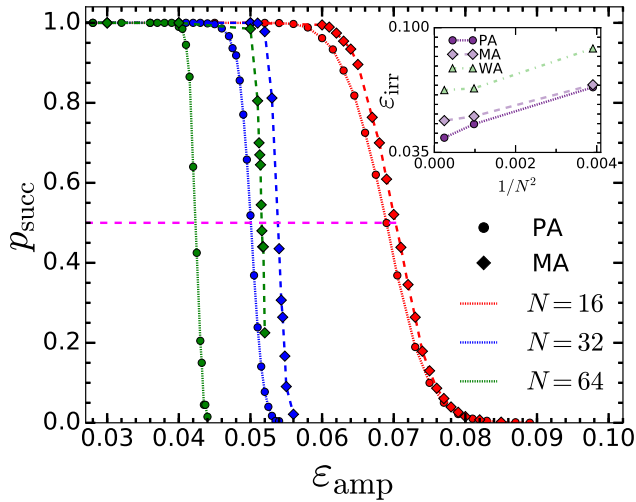
FIG. 6. Success rate p_{\text{succ}} of the convergence to a limit cycle under cyclic shearing at amplitude \epsilon_{\text{amp}} . Shown are results for ensembles of poorly-aged (circles) and moderately-aged (diamond) glasses with system sizes N = 16 (red), 32 (blue), and 64 (green). Intersections with the dashed horizontal line indicate strain amplitudes where the probability of finding a limit-cycle is 1/2 . Inset: The plot of strain amplitudes \epsilon_{\text{irr}} at which p_{\text{succ}} = 1/2 against 1/N^2 for the poorly-, moderately-, and well-aged glasses, PA, MA and WA.
