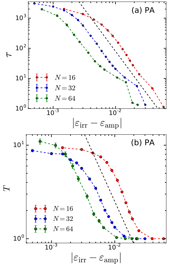
FIG. 7. Convergence to limit cycles of poorly-aged (PA) glasses: (a) Duration \tau of transients vs. relative cycle amplitude |\epsilon_{\text{irr}} - \epsilon_{\text{amp}}| , where \epsilon_{\text{irr}} is the system size dependent strain amplitude where the success-rate p_{\text{succ}} of cyclic response is 1/2 , cf. Fig. 6. The dashed line is a power-law with exponent 2.7 and serves as a guide to the eye. (b) The period T of the cyclic response in units of the number of driving cycles for the poorly-aged samples at different system sizes. The dashed line is a power-law with exponent 1.5 and serves as a guide to the eye.
