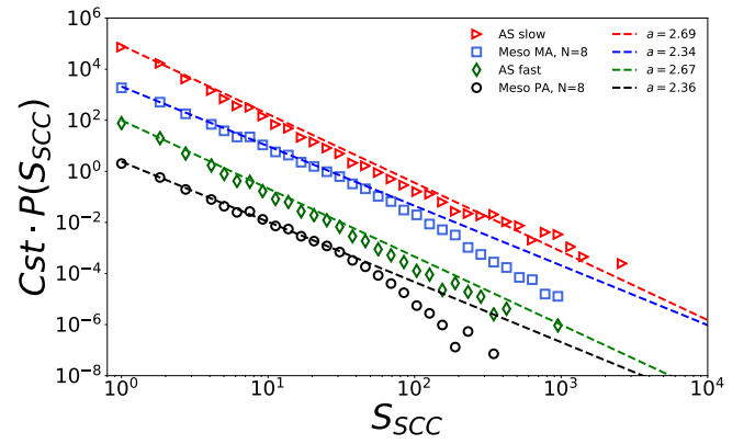
FIG. 13. Comparison of the SCC distribution obtained from the atomistic simulations with those obtained from a mesoscopic model with compatible system size N = 8 . Shown are the distributions for poorly- and medium-aged glasses.
