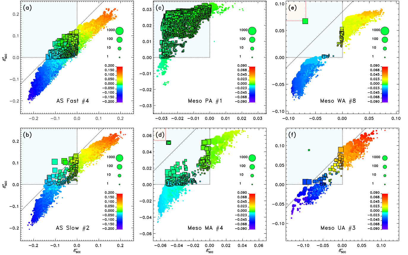
FIG. 11. The coarse-grained disorder-landscape, atomistic vs. mesoscopic models, and the effect of aging – The six panels show the scatter plots of the SCCs found in catalogs obtained from atomistic (first column) and our N = 32 mesoscopic simulations (second and third columns). Panels (e) and (f) depict the disorder landscape extracted from increasingly better-aged samples of the mesoscopic model. Each symbol represents an SCC, while the size and color correspond to the size of the SCC and the average plastic strain \varepsilon^{\text{pl}} of the mesostates constituting that SCC. Each SCC has at least one U - and one D -transition that leads to another SCC, and we denote by \varepsilon_{\text{SCC}}^{\pm} the threshold strains to trigger these transitions. As explained in the text, taking the extremes of these exit strains, the corresponding interval (\varepsilon_{\text{SCC}}^-, \varepsilon_{\text{SCC}}^+) provides a range of strain values over which the system will be trapped in that SCC. These strains are used as coordinates for placing the SCC in the plot. Box-shaped symbols indicate that the SCC supports at least one cycle under symmetric cyclic shearing. The area shaded in red in panels (d) and (e) indicates where cycle supporting SCCs would have to be located if they were to contain cycles at strain amplitudes beyond the onset of the irreversibility transition, as obtained from the inset of Fig. 6. For panels (c) and (f) this region lies outside the plot window. The diagonal dashed lines corresponds to the average SSC strain range of Eq. F1, estimated as \varepsilon_{\text{SCC}}^+ - \varepsilon_{\text{SCC}}^- = \Sigma_{\text{ss}}/\mu , where \Sigma_{\text{ss}} is the steady-state stress under monotonous strain loading. Refer to text for further details.
