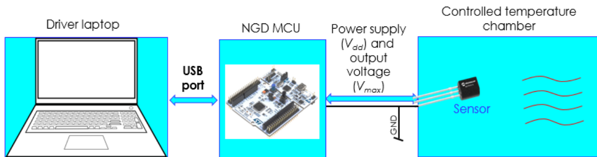
FIGURE 1. Configuration of real-time anticipated temperature test based on heated sensor configuration.
