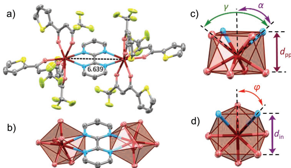
Figure 3. Single-crystal X-ray structure of [L_2(Yb(tffa)_3)_2] (ellipsoids are plotted at the 50% probability level, and H atoms and disorder are omitted for clarity, CCDC 2209638): a) full structure, b) polyhedral view of the Yb_2 coordination environment, c) polyhedral view of Yb environment, and d) view along the pseudo- S_8 axis.
