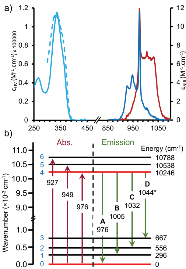
Figure 5. a) Absorption spectra in the UV (blue solid line, 5.75 \times 10^{-6} M) and NIR (dark blue, 4.4 \times 10^{-3} M) ranges and normalized excitation (blue dashed lines, \lambda_{\text{exc}} = 980 nm) and emission (red line, \lambda_{\text{em}} = 336 nm) spectra of the [\text{L}_2(\text{Yb}(\text{tffa})_3)_2] complex in \text{CH}_3\text{CN} . b) Energy diagram for [\text{L}_2(\text{Yb}(\text{tffa})_3)_2] , where each horizontal line represents a Kramer's doublet (* denotes a transition determined computationally).
