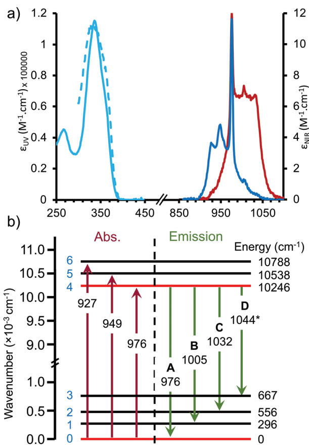
Figure 5. a) Absorption spectra in the UV (blue solid line, 5.75 \times 10^{-6} m) and NIR (dark blue, 4.4 \times 10^{-3} m) ranges and normalized excitation (blue dashed lines, \lambda_{\text{em}} = 980 nm) and emission (red line, \lambda_{\text{exc}} = 336 nm) spectra of the [\text{L}_2(\text{Yb}(\text{ttfa})_3)_2] complex in \text{CH}_3\text{CN} . b) Energy diagram for [\text{L}_2(\text{Yb}(\text{ttfa})_3)_2] , where each horizontal line represents a Kramer's doublet (* denotes a transition determined computationally).
