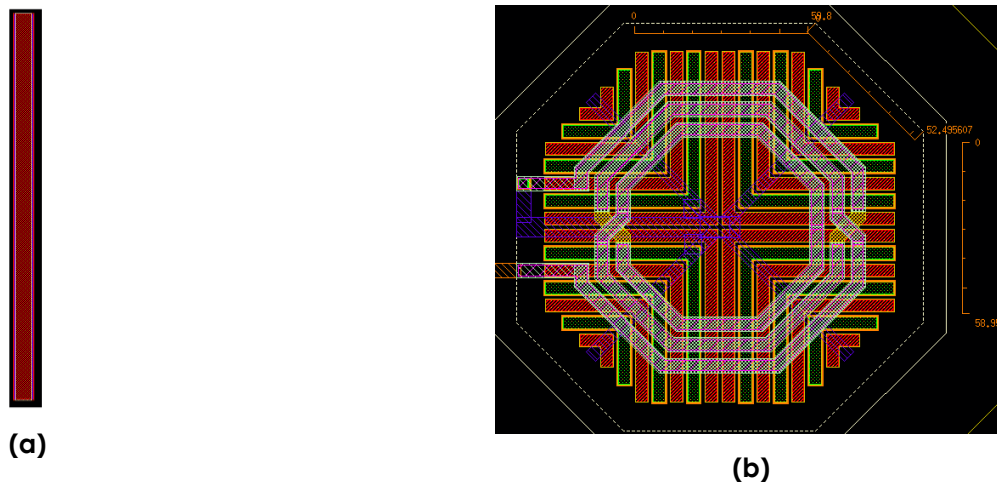
Fig. 6. LP-NGD circuit (a) resistor and (b) inductor die.
