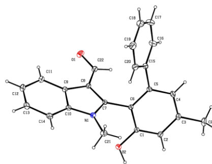
Figure 1: Crystal Structure of 3a (CCDC No. 2217042)
