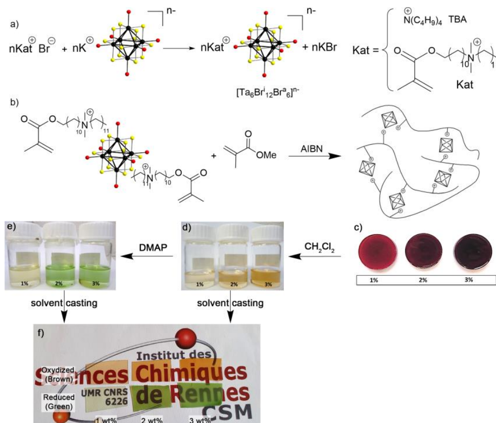
Figure 2. (a) Representation of the cationic metathesis reaction between organic ammonium cations (Kat) and potassium in K_4[(Ta_6Br^i_{12}Br^a_6)] , (b) Representation of the bulk radical polymerization reaction with MMA carried out at 60 °C for 24 h, (c) the brown pellets obtained, (d) Solution of brown pellets in CH_2Cl_2 , (e) Reduction in brown Ta 6 cluster units in solution with two equivalents of DMAP and (f) Pictures of brown and green films obtained by solvent casting.
