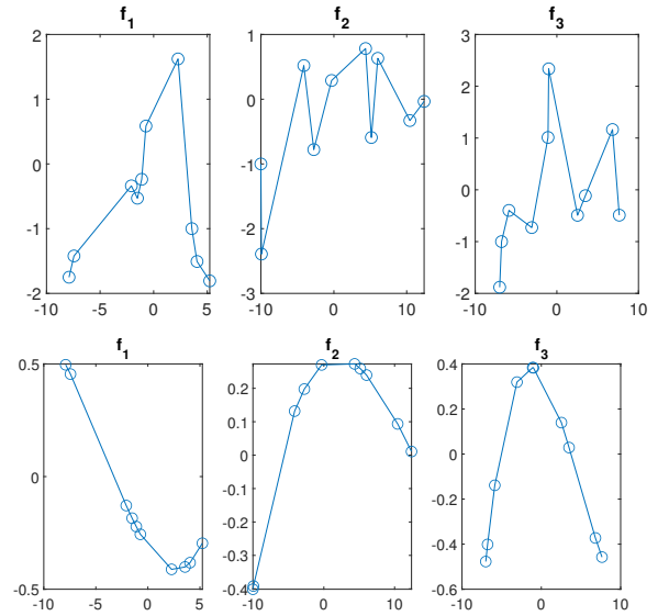
Fig. 3. Due to the presence of slice ambiguities, recovering the functions \mathbf{g} and \mathbf{h} from the PTD requires additional attention. Plot of the estimation of \mathbf{h} without (top) and with (bottom) slice ambiguity correction.
