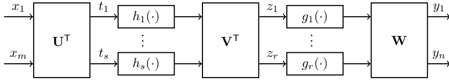
Fig. 2. Decoupled representation of \mathbf{f} into a two-layer model, as in (13). This naturally leads to a PT decomposition of the corresponding Jacobian tensor.
