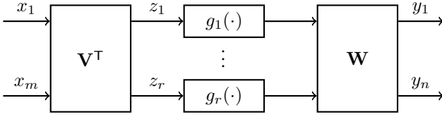
Fig. 1. Decoupled representation of \mathbf{f} into a single-layer model as in (12). This naturally leads to the CPD of the corresponding Jacobian tensor.
