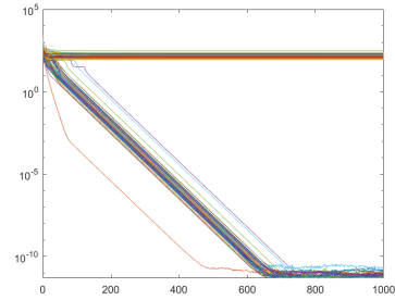
Fig. 4. The convergence plot shows a linear convergence to an error of order 10^{-10} in 46 out of 100 random initializations.
