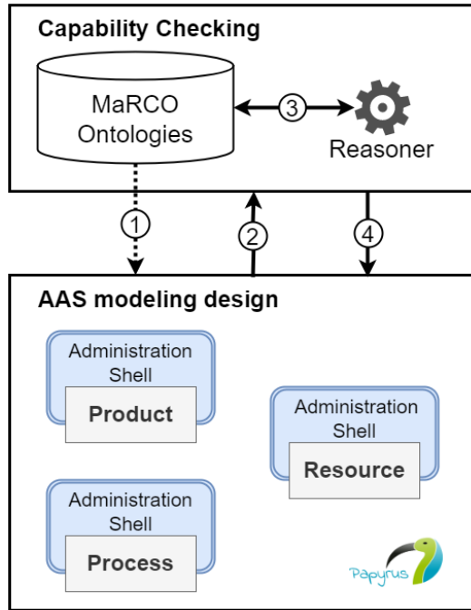
Figure 3: Capability checking architecture
