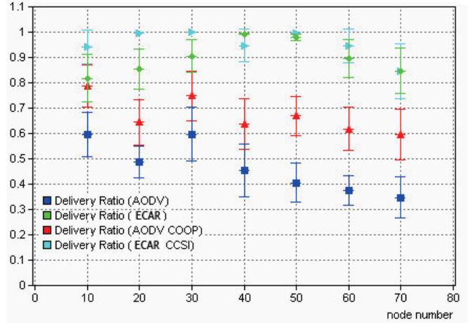
Fig. 5. Delivery Ratio VS Number of nodes
