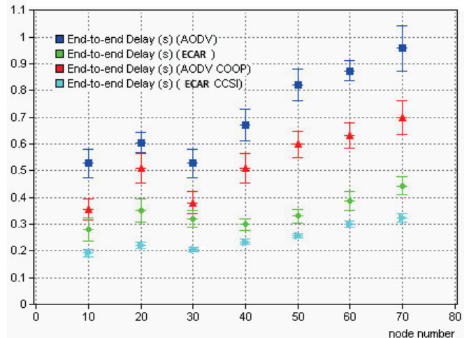
Fig. 6. End-to-End delay VS Number of nodes
