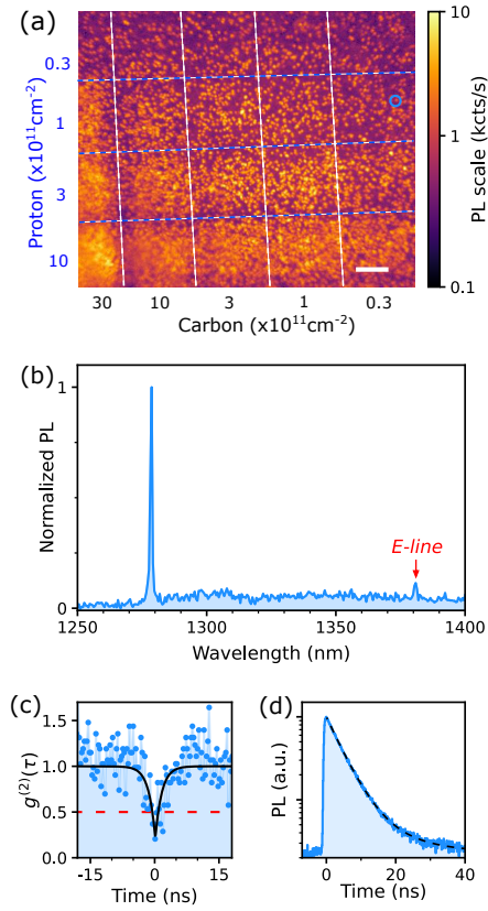
FIG. 3. (a) PL map of the SOI sample # 1 in the region of low irradiation fluences. The vertical white (horizontal blue) dashed lines are guides for the eyes splitting the stripes with different carbon (proton) fluences, whose value is indicated in the bottom (left) axis. The white bar scales for 10 \mu\text{m} . (b) PL spectrum detected for an isolated G center indicated by the blue circle in (a). (c) Corresponding intensity-correlation function g^{(2)}(\tau) , without any correction from background or detector noise counts. The photon antibunching with g^{(2)}(0) < 0.5 evidences the emission of single photons. These data are recorded at 30 K under excitation at 532 nm with an optical power of 10 \mu\text{W} . (d) Time-resolved PL trace for this single G center acquired with a 150 ps 532 nm pulsed laser.
