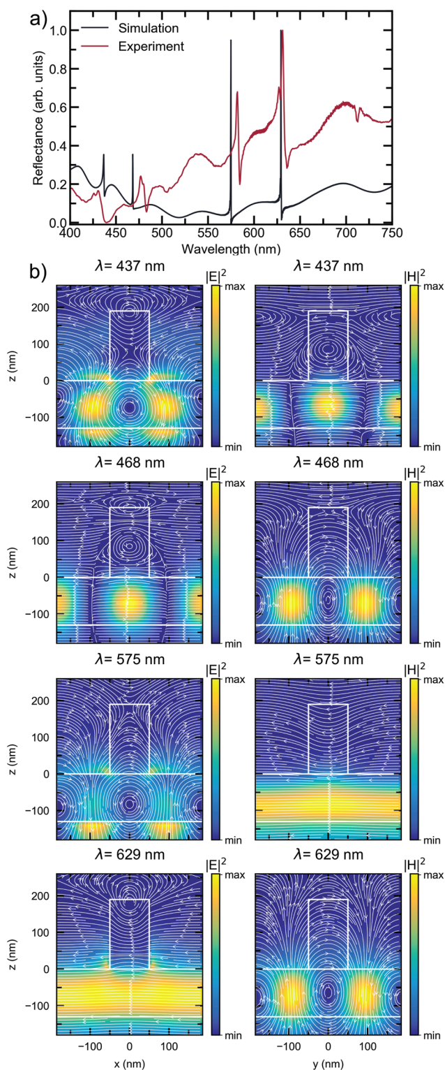
Figure 4. a) Comparison between the measured reflection spectrum (red curve) and the spectrum simulated by FDTD calculations (black curve). b) Electric (left column) and magnetic (right column) field intensity distributions and current loops (white arrows). The maps, acquired at the wavelength of the peaks of the black curve in panel (a), are reported in order of increasing wavelength from top to bottom. The shape of the nanopillar and the boundaries of the residual layer are indicated with the white lines.
