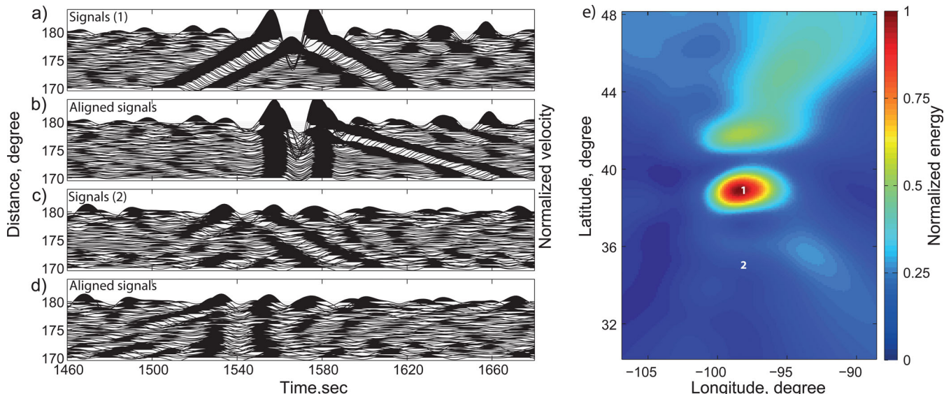
Figure 7. (a) Seismograms bandpassed between 20 and 50 s, stacked in 1^\circ bins, and aligned with respect to distances to the epicentre's antipode. (b) Similar to (a) after applying a moveout correction with a slowness of PP waves propagating along the minor arc. (c) Similar to (a) but aligned with respect to point 2. (d) Similar to (c) and after applying a moveout correction maximizing the function from eq. (3). (e) Normalized beamforming result obtained from eq. (2) over an area around the antipode for the minor waves of PP . White numbers indicate positions of points 1 and 2 discussed in the text.
