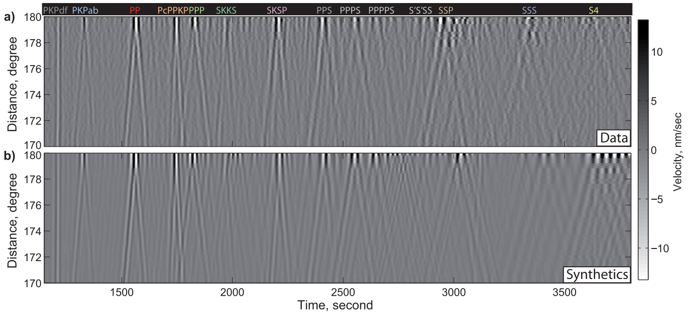
Figure 5. Time-distance gathers computed with averaging vertical-component seismograms in 0.25° bins. Signals were bandpassed between 20 and 50 s. (a) Observations. (b) Synthetics.
