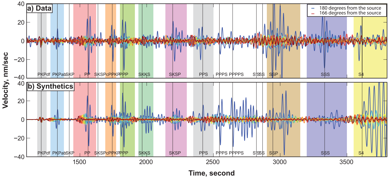
Figure 4. Vertical component seismograms bandpassed between 20 and 50 s and averaged in 1° distance bins. (a) Observations. (b) Synthetics. The colours of traces correspond to the distance from the source and evolve from red (166°) to blue (180°).
