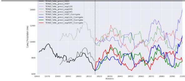
Figure 2 : Temporal evolution of annual precipitation (in mm) and average temperatures (in °C) over the historical period 1981-2014 (in black) and future (SSP126 in blue, SSP245 in green and SSP585 in red) before (dotted lines) and after correction of the biases (solid lines) of the model on South West Coast
