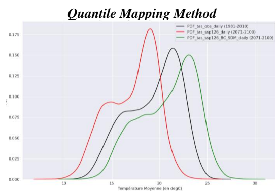
Figure 1 : PDF of mean annual temperatures (°C) for the Fianarantsoa station: Observation in black, the raw output of the ALADIN model (in red), and the ALADIN model corrected (in green)
