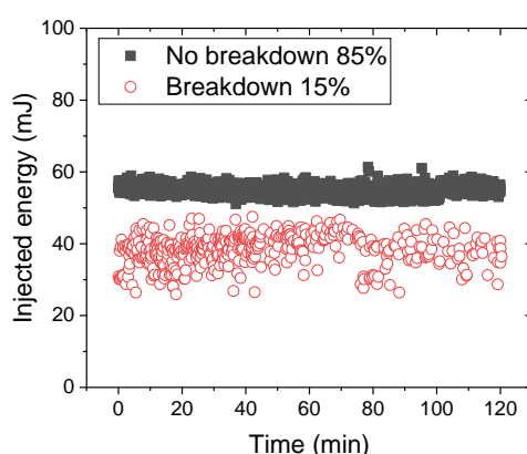
Figure 3. Time evolution of the injected energy per pulse for pin-to-pin discharges in Cr(VI) solution (47 mg/L, \sigma=4 mS/cm, pH=2.3), V = 100 mL, U=9 kV, \Delta t = 500 \mu s, gap = 2 mm, electrodes length = 0 \pm 10 \mu m, f = 50 Hz.
