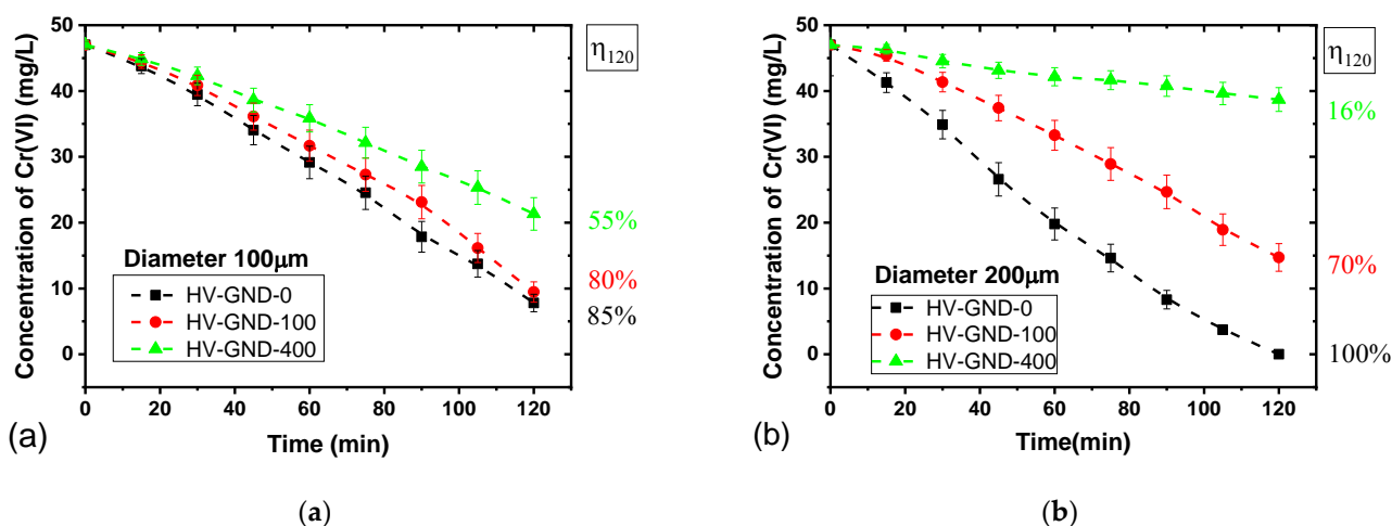
Figure 5. Concentration of Cr(VI) as a function of time for different electrodes lengths (0, 100, 400 \mu\text{m} ) and for two diameters: (a) \varnothing = 100 \mu\text{m} and (b) \varnothing = 200 \mu\text{m} obtained during for pin-to-pin discharges in Cr(VI) solution (47 mg/L, \sigma=4 \text{ mS/cm} , \text{pH}=2.3 ), V = 100 \text{ mL} , U = 9 \text{ kV} , f = 50 \text{ Hz} , \Delta t = 500 \mu\text{s} , gap = 2 mm. \eta_{120} refers to the reduction efficiency after 120 min of PLI process.
