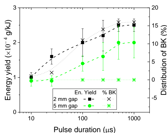
Figure 9. Energy yield and breakdown distribution according to the pulse duration for pin-to-pin discharges in Cr(VI) solution (47 mg/L, \sigma=4 mS/cm, pH=2.3) – U=9kV, V = 100 mL, electrodes length = 0\pm10 \mu m , f = 50 Hz.
