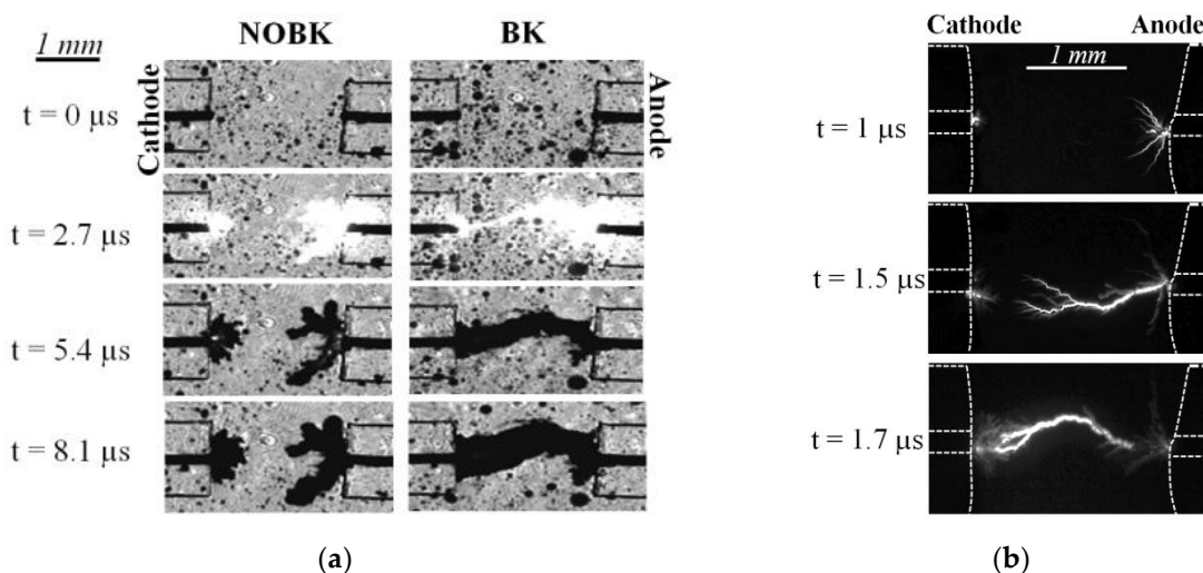
Figure 4. Optical diagnostics of pin-to-pin discharges in Cr(VI) solution (47 mg/L, \sigma=4 mS/cm, pH=2.4) \Delta t=500 \mu\text{s} , gap = 2 mm, electrodes length = 0\pm 10 \mu\text{m} . (a) Time-resolved shadowgraphy of case NOBK and case BK ( U=11 kV; exposure time = 0.37 \mu\text{s} ); (b) Fast imaging for three successive BK experiments ( U=12.5 kV, exposure time = 100 ns).
