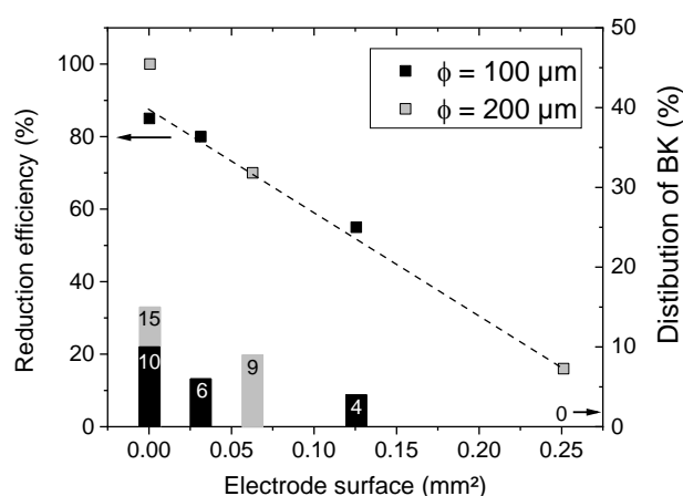
Figure 6. Reduction efficiency (dots) and Distribution of BK (columns) after 120 minutes according to the electrode surface in contact with liquid.
