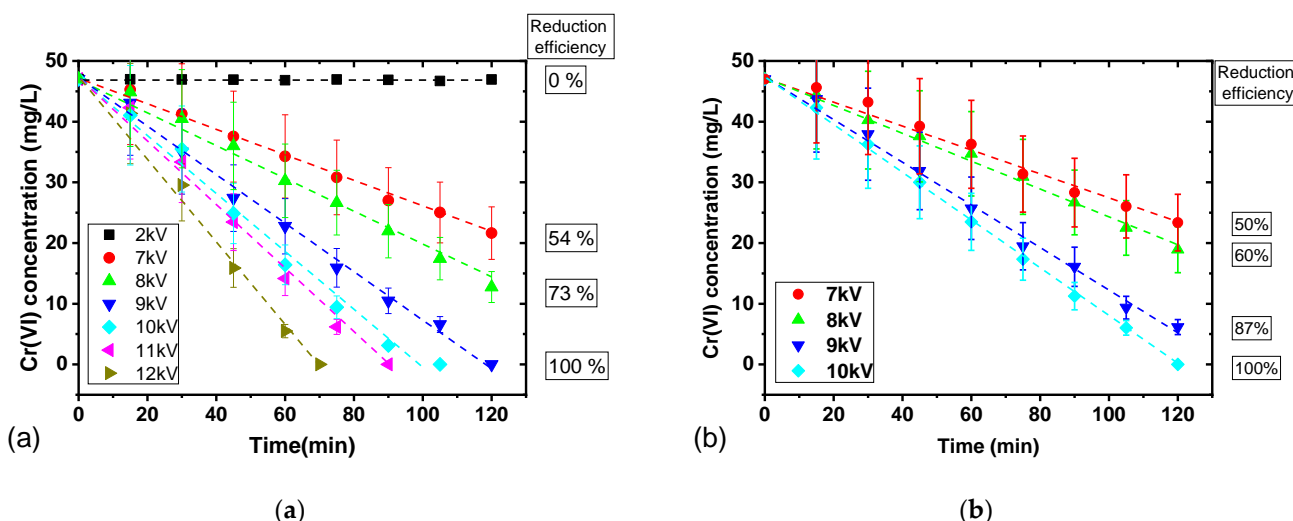
Figure 7. Time evolution of Cr(VI) concentration according to the applied voltage for (a) 2 mm gap and (b) 5 mm gap obtained during pin-to-pin discharges in Cr(VI) solution (47 mg/L, \sigma=4 \text{ mS/cm} , \text{pH}=2.3 ) V = 100 \text{ mL} , \Delta t = 500 \mu\text{s} , electrodes length = 0 \pm 10 \mu\text{m} , f = 50 \text{ Hz} .
