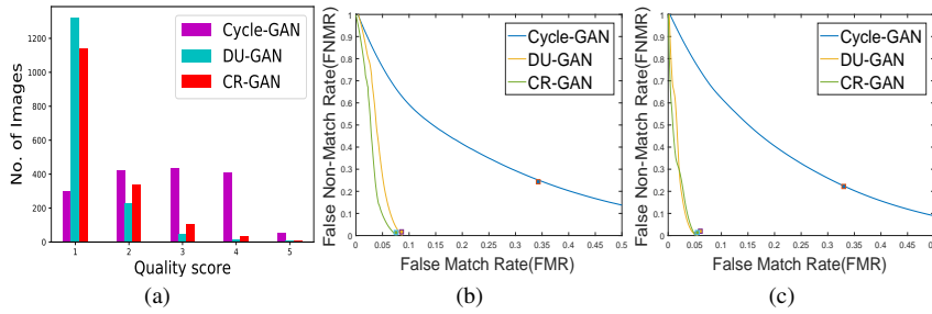
Fig. 15 Comparison of the proposed CR-GAN with state-of-the-art generative adversarial network based fingerprint enhancement models Cycle-GAN and DU-GAN on the Rural Indian Fingerprint database: (a) histogram of NFIQ scores; DET curves obtained using (b) Bozorth (c) MCC
