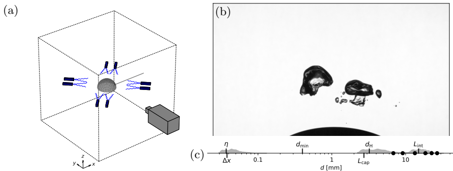
Figure 2: The experiment on large cavity disintegration. (a) Schematic of the experiment. Air is bubbled into an inverted hemispherical cup located just under the convergence of the turbulent jets, and the cup is rapidly rotated to expose the air to the turbulence. The experiment is lit from behind (not shown) and filmed with a high-speed camera. (b) One representative image of a cavity breaking apart, with the cup still slightly visible at the bottom of the image. (c) The characteristic length scales \eta , d_H , L_{\text{cap}} , and L_{\text{int}} taken in analyzing the data, the pixel size \Delta x and the minimum bubble size considered d_{\text{min}} , and the diameters of the air cavities studied (circles). Distributions of the turbulence quantities in the field of view in the center of the tank (within the green rectangle in Figure 1) are also given in gray.
