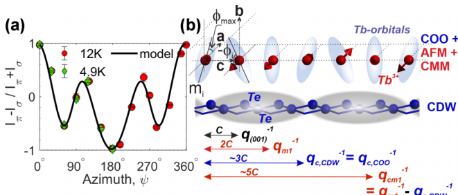
FIG. 4. (a) Azimuthal dependence of q_c measured above and below the magnetically ordered state in zero field. Black solid line is the simulation as described in the text and SM [28]. (b) The schematic of the periodicities of COO (represented by local quantization axis— m_i of the Tb-4 f orbitals, blue ellipsoids) with tilt angle \phi_i about the crystalline a axis, AFM and CMM of the Tb 3+ spins (red arrows) in the Tb-Te layer which follow the CDW (gray clouds) periodicity set in the Te-Te layer of TbTe 3 .
