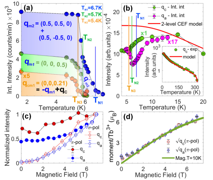
FIG. 3. (a) Temperature evolution of magnetic peaks q_{m2} , q_{m1} , and q_{cm1} measured with neutron diffraction indicating three consecutive magnetic transitions. (b) The scaled temperature dependence of the COO peaks q_a and q_c from the resonant x-ray scattering manifesting a reduction of intensity in the magnetically ordered state. Inset: the temperature dependence of q_c upon approaching the CDW transition. Solid red lines are the simulated temperature evolution of q_c based on the thermal population of a two-level crystal electric field split (by 4.5 meV) Tb- 4f state [28]. (c) Magnetic field dependence of the magnetic ( \pi -pol) and orbital ( \sigma -pol) contributions to the COO peaks q_a and q_c measured in the paramagnetic state at 10 K. All the intensities are normalized to their value at 7 T. (d) Square root of the magnetic ( \pi -pol) intensities as a function of field arbitrarily scaled to match the magnetization of a single crystal of TbTe_3 along the b axis measured at 10 K.
