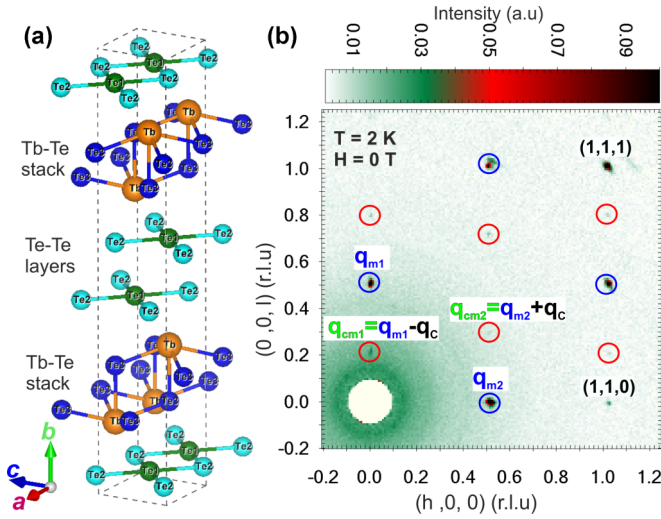
FIG. 1. (a) Unit cell of \text{TbTe}_3 where the two-dimensional Te-Te sheets sandwich the Tb-Te stacks. (b) Neutron diffraction map for the single crystal of \text{TbTe}_3 measured at E2 diffractometer in the a - c plane at T = 2 K with intensities as indicated in the colorbar. The intensities are integrated over the out-of-plane b axis and reveal CMM peaks with propagation vectors q_{\text{cm}1} = (0, 0, 0.21) , q_{\text{cm}2} = (0.5, 0.5, 0.29) (red circles) and AFM peaks q_{\text{m}1} = (0, 0, 0.5) , q_{\text{m}2} = (0.5, 0.5, 0) (blue circles).
