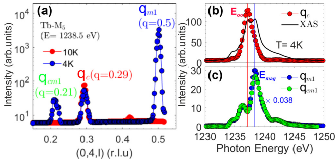
FIG. 2. Soft x-ray resonant diffraction peaks measured at UE46-PGM1 beamline: (a) show the COO- q_c , CMM- q_{cm1} and AFM- q_{m1} peaks along the c -axis measured at T = 4 K below T_{N3} = 5.4 K. The resonance profile, (b) of the COO peak at fixed- Q plotted against the Tb- M_5 absorption edge (black solid line), indicating a maximum at E_{oo} = 1237.3 eV, and (c) of the magnetic peaks featuring a distinctly different multi-peak profile with a maximum at E_{mag} = 1238.5 eV. All other lines are guides to the eye.
