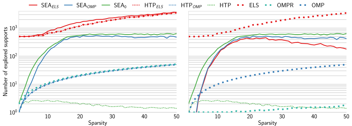
Figure 11: Left: Average number of explored supports by algorithms solving the 200 problems in Section 5.2, across sparsity levels k \in [1, 50] . Right: Average number of explored supports from algorithms initialization in the same setup.
