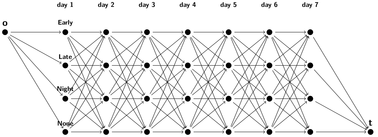
Figure 1: Example of a roster graph network. Here, the horizon includes 7 days and \mathcal{S} = \{\text{Early}, \text{Late}, \text{Night}, \text{None}\} .
