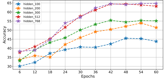
(a) Linear evaluation for models trained with different choices of number of hidden layers and epochs.
