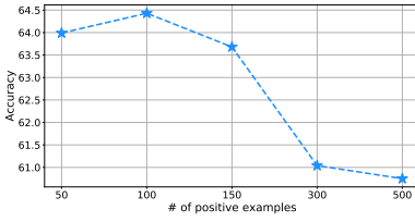
(a) The effect of the number of positive examples.
