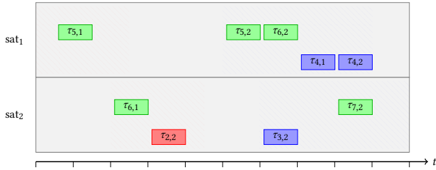
Figure 2: A solution schedule for example in Figure 1.
