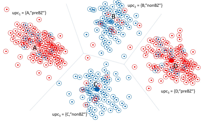
Figure 4. Universal Prediction Clusters (UPC) - Each dot is a sentence processed in the learning phase (Red: Pre-Bug-Zone, Blue: Random-Zone)
