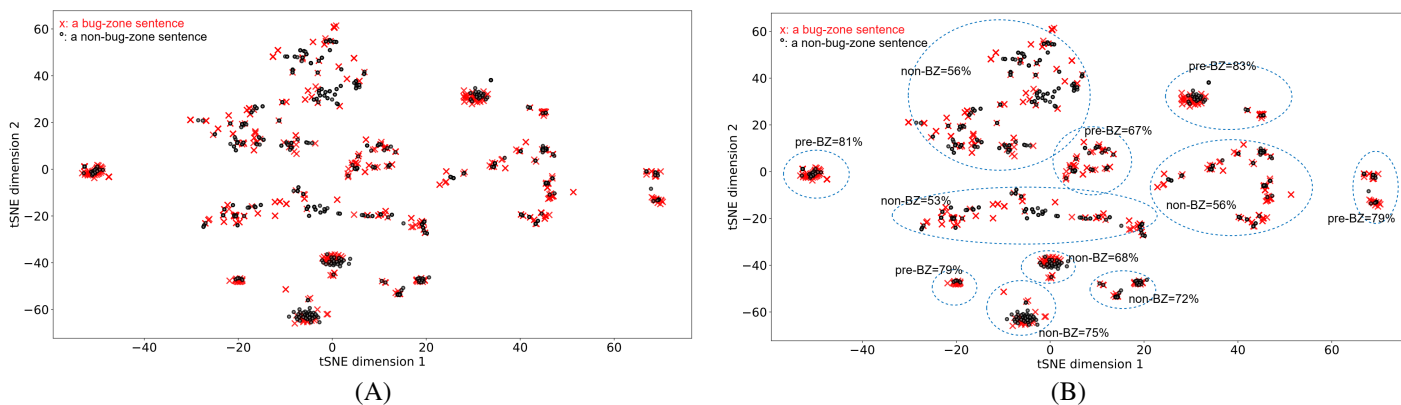
Figure 6. (A) A projection of Pre-Bug-Zones and Random-Zones vectors in 2D from the telecom case study, (B) UPCs created from telecom case study
