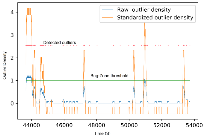
Figure 8. Outlier density curve for the Train Ticket benchmark. The detected outlier shows in red dots and the threshold line in green.
