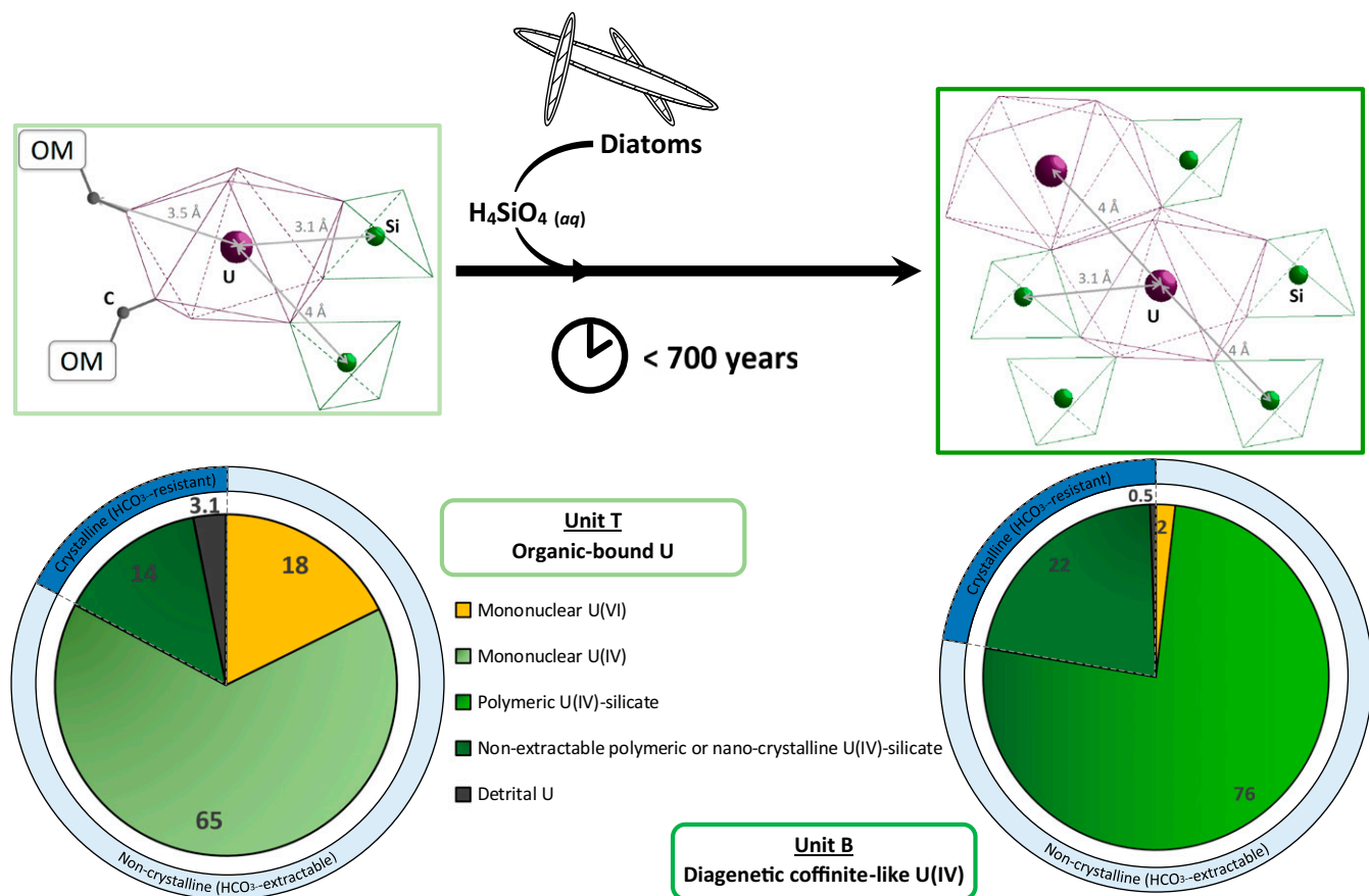
Fig. 3. Conceptual model of the observed natural U transformation: Noncrystalline U(IV) (Unit T, Left ) transforms to U(IV)–silica polymers/nanocrystalline coffinite ( U^{IV}SiO_4 \cdot nH_2O ) (Unit B, Right ) in less than 700 y in Lake Nègre sediments. This transformation is enhanced by diagenetic remobilization of Si, potentially from diatoms. Tentative models of molecular structure around U in the investigated samples are shown in boxes on the top; U atoms are represented in purple and Si (and/or P in Unit T) atoms in green; “OM” indicates organic matter-bound monodentate C neighbors (in gray). Coordination polyhedra to first oxygen ligands are drawn as thin lines. For Unit T, corner linkage to organic carbon (3.5 Å) in addition to U–Si and/or U–P contributions. For Unit B, short-range coffinite-like cluster with U–Si edge-sharing linkage ( \sim 3.1 Å) and slightly elongated distances ( \sim 4 Å) for edge-sharing U–U and corner-sharing U–Si linkage. Pie charts display resulting repartitions of crystalline and noncrystalline U fractions according to 1 M bicarbonate extraction ( SI Appendix, Supplementary Text and Fig. S23 ), with uncertainties (2SD) between 3 and 4%. Gradation in the green color indicates an increase in the degree of polymerization of U(IV)–silica species.
