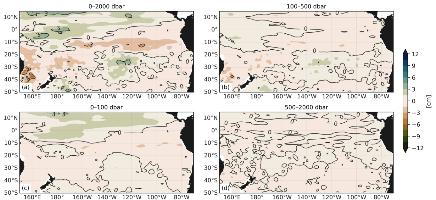
Figure 4. Differences in the Roemmich-Gilson Argo-based halosteric sea level (HSL) for 2016 minus 2014 over (a) 0–2000 dbar, (b) 100–500 dbar, (c) 0–100 dbar and (d) 500–2000 dbar. Contour lines (see inline numbers for HSL intervals) are also shown.
