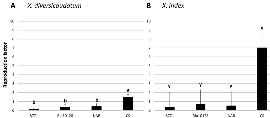
FIGURE 2. Reproduction factors (RFs) of X. diversicaudatum (A) and X. index (B) in the F1 accession 8771, the BC1 accession NAB, the X. index susceptible control accession CS and the X. index resistant control accession Rip10128. Data are means ( \pm SE) of 7 replicates (8771, NAB and CS) and 5 replicates (Rip10128) for X. diversicaudatum and of 5 replicates (all accessions) for X. index . Bars with different letters significantly differ according to the Fisher LSD test ( P \leq 0.05 ).
