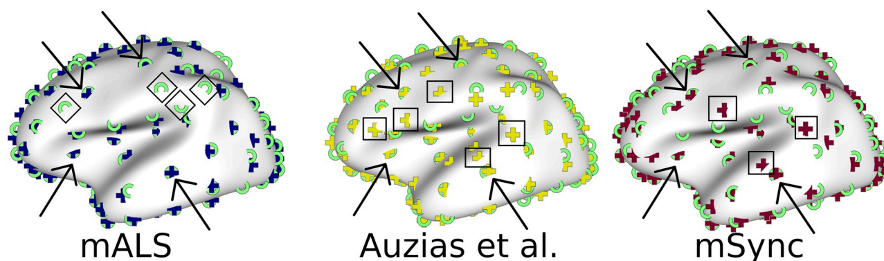
Fig 9. Superimposition of the centroids from mALS, Auzias et al., and mSync shown as crosses with those of Kaltenmark et al. shown as green rings. mSync is representative of the methods kerGM, MatchEig and CAO that also result in 101 clusters. The arrows point to centroids that are robust across methods. The squares indicate centroids corresponding to small clusters located on gyri. Diamonds indicate centroids that differ between mALS and Kaltenmark et al..
