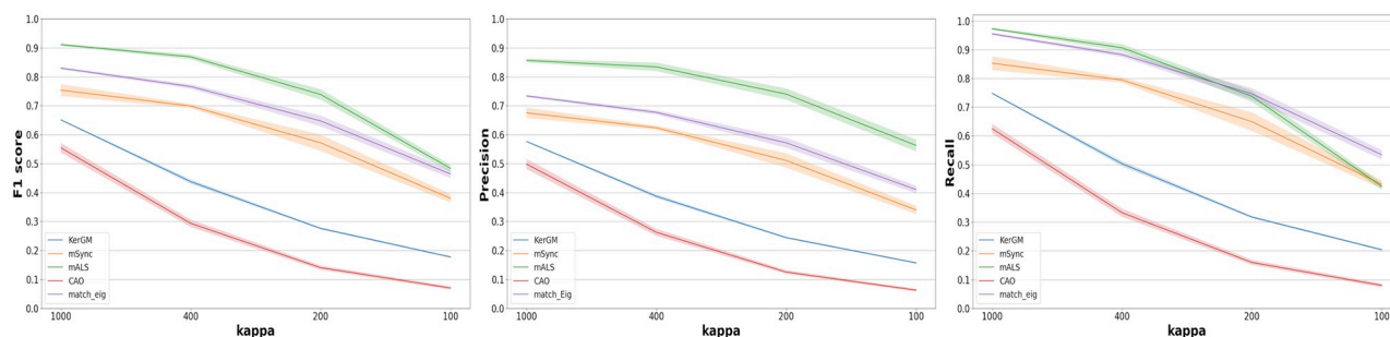
Fig 4. F_1 -score, precision and recall for \kappa \in [1000, 400, 200, 100] . For each method, we plot the average across the 10 simulated populations as a line and the standard deviation as the shaded region of the same color.
