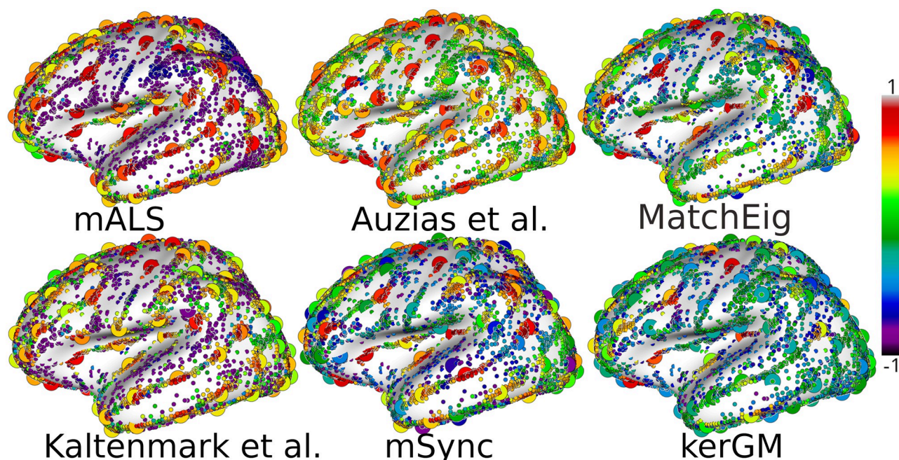
Fig 6. For each method, we show the silhouette coefficient of each node from every graphs, as well as corresponding centroids as larger circles. Each centroid (larger circles) is colored according to the average of the silhouette coefficient of corresponding nodes.
